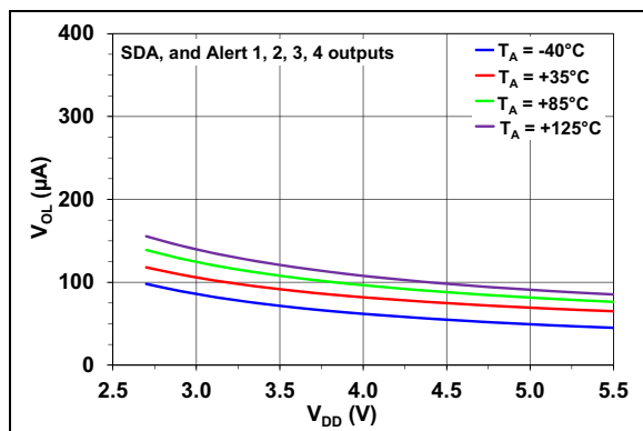
FIGURE 2-21: SDA and Alert Outputs, V_{OL} Across V_{DD} .
