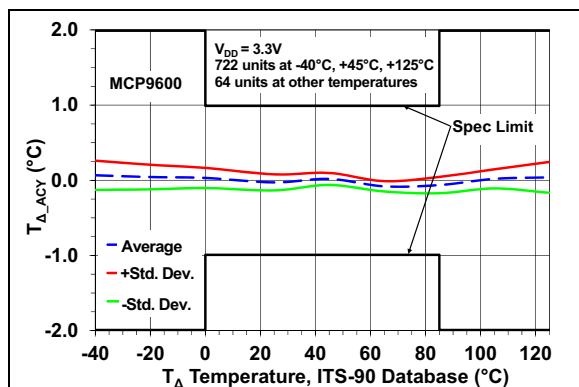
FIGURE 2-20: Cold-Junction Sensor Temperature Accuracy.
