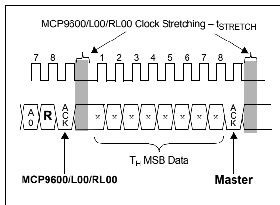
FIGURE 4-2: Clock Stretching.
