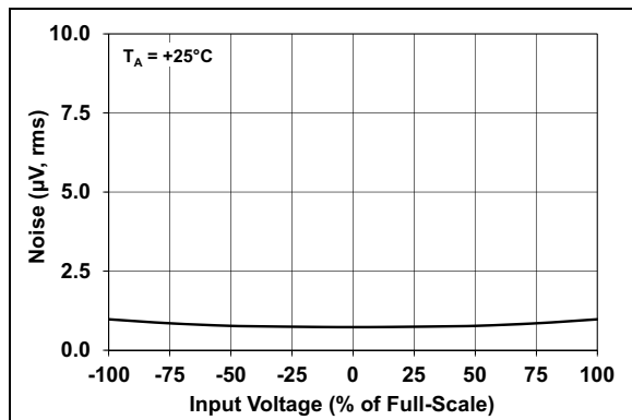
FIGURE 2-19: Input Noise, % of Full Scale.
