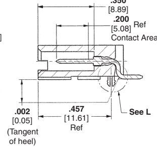
Section K-K
