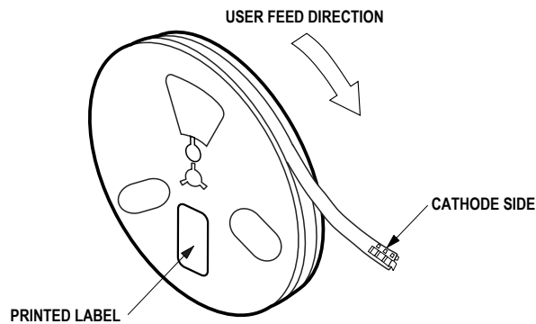
Figure 9. Reeling Orientation.
