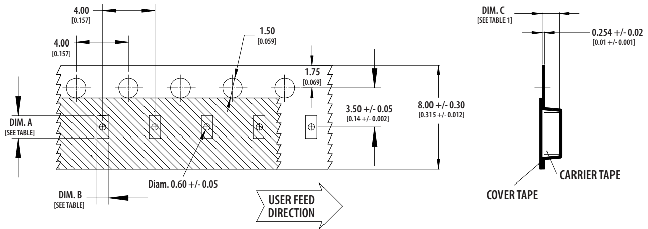
Figure 8. Tape Dimensions.
