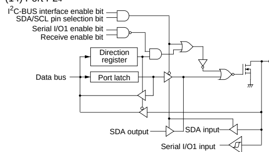
(14) Port P24
