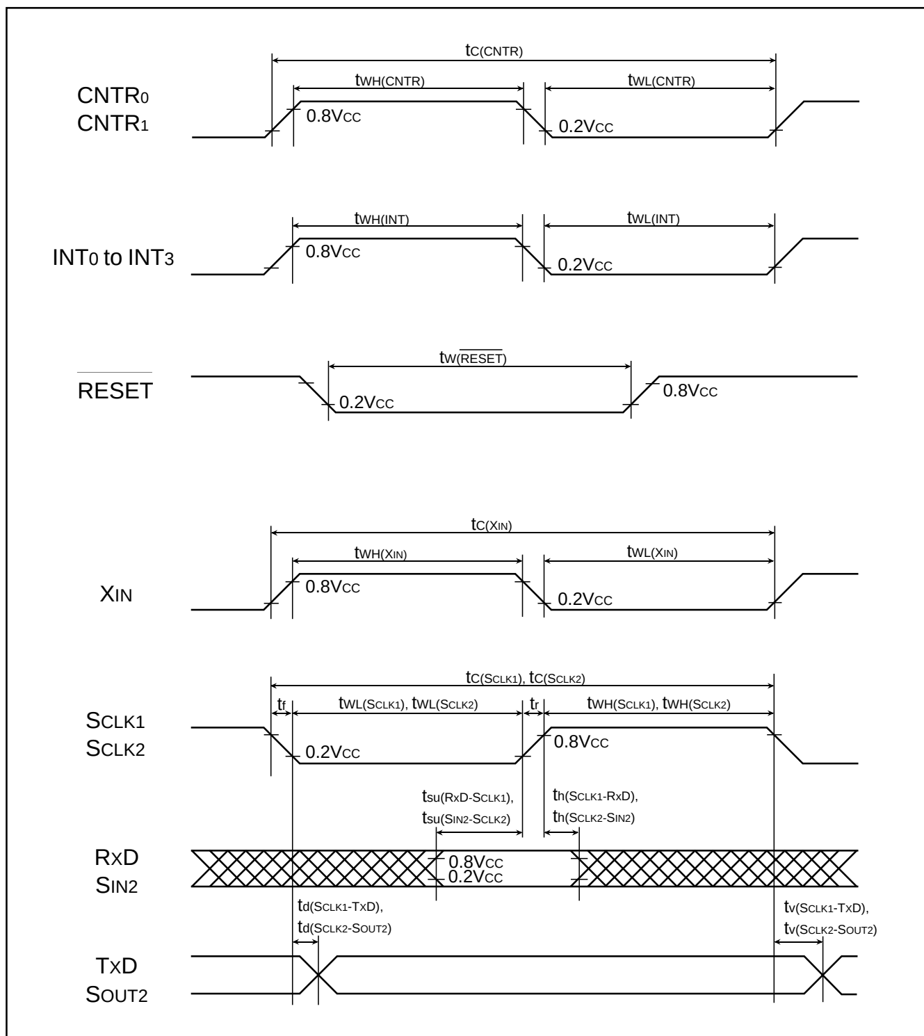
Fig. 84 Timing diagram
