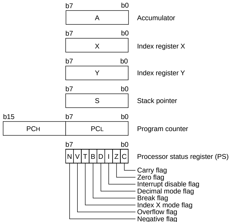
Fig.4 740 Family CPU register structure
