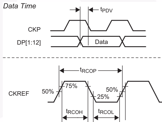
Figure 10. Deserializer Data Valid Window Time and Clock Output Parameters
