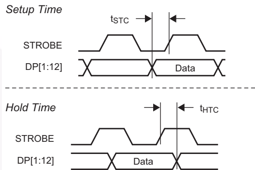
Figure 8. Serial Setup and Hold Times
