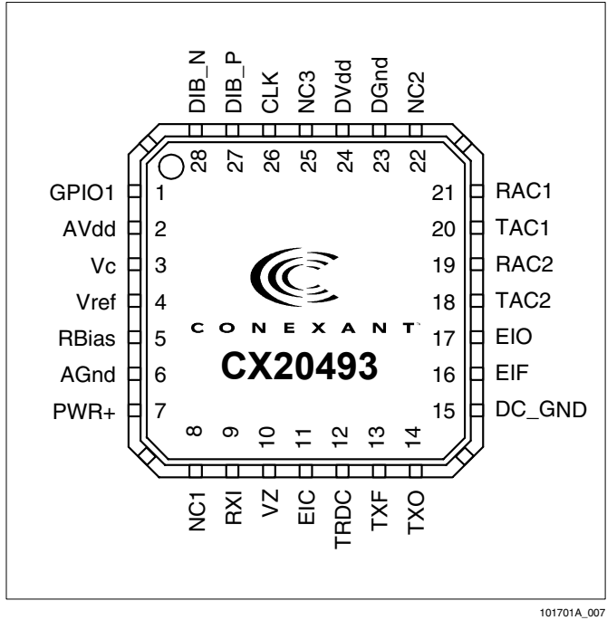
Figure 3-6. CX20493 LSD 28-Pin QFN Pin Signals
