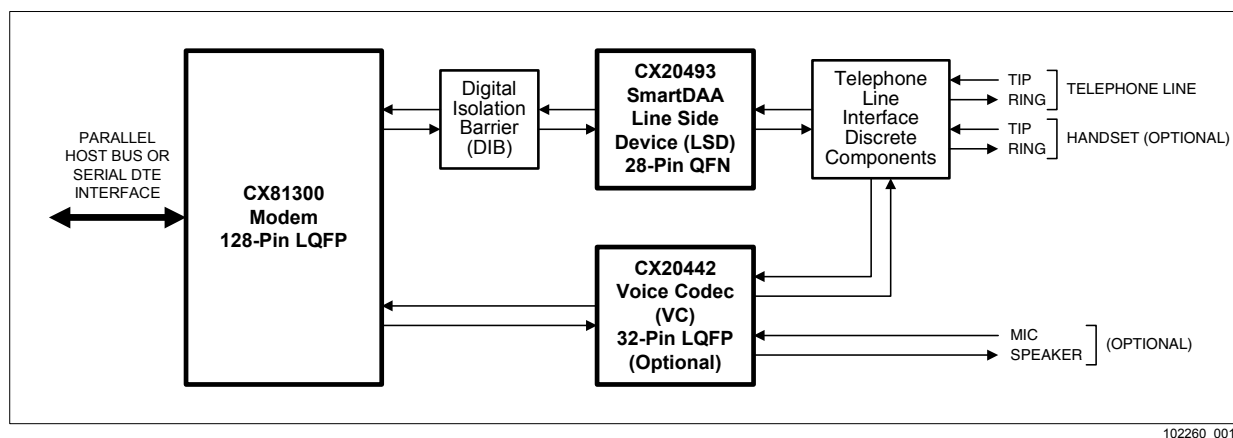
Figure 1-1. SmartACF Modem Simplified Interface Diagram
