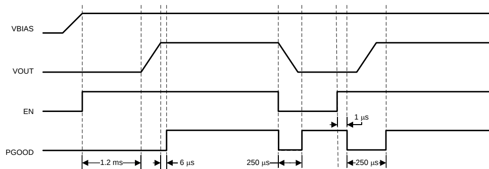
Figure 11. Power Good Operation
