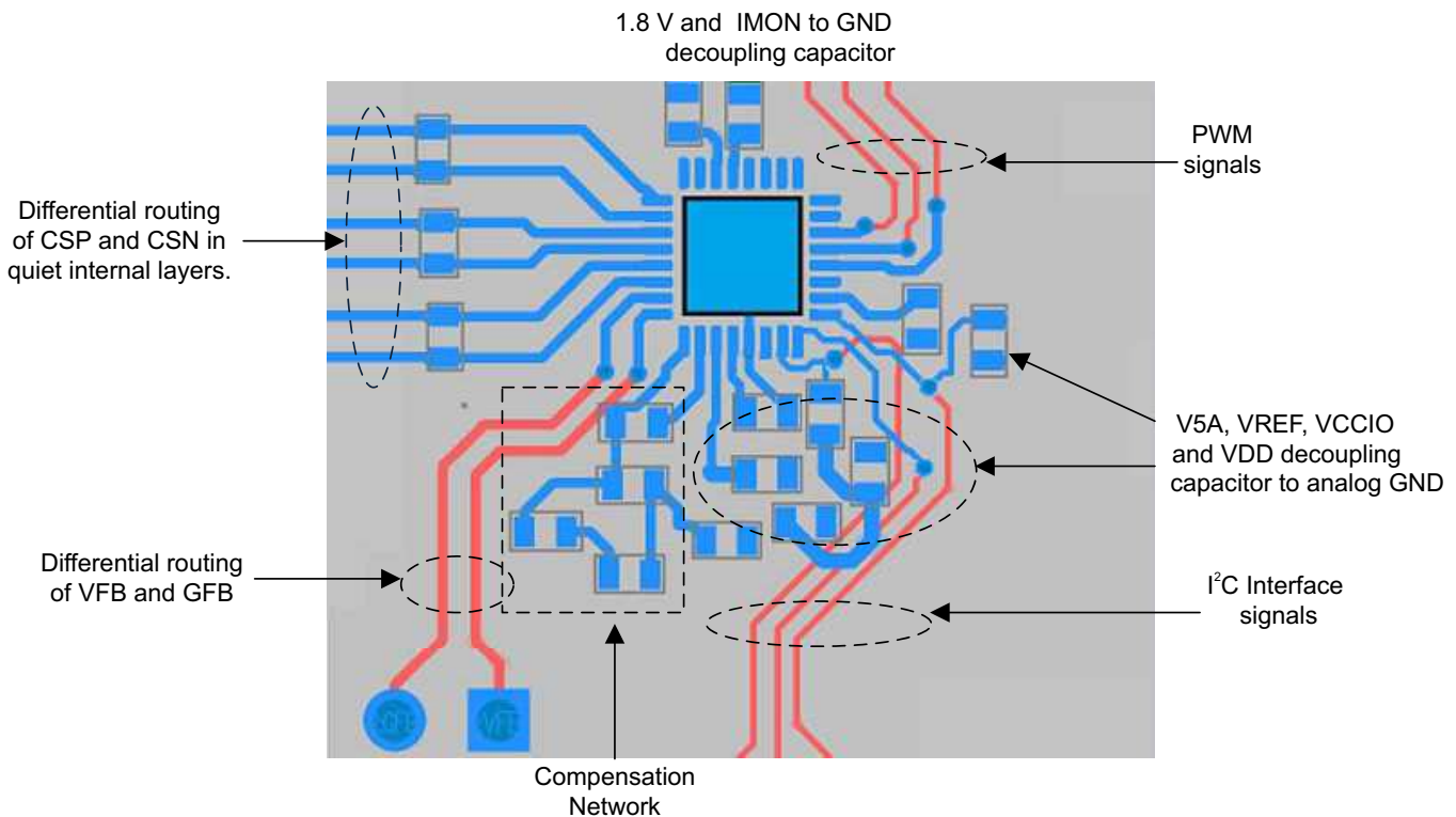
Figure 22. Example Layout
