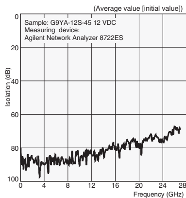
High-frequency Characteristics (Isolation)
