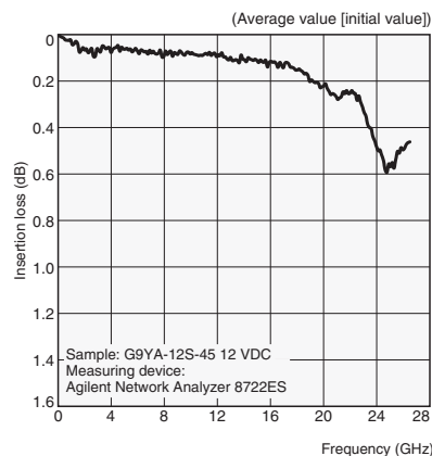
High-frequency Characteristics (Insertion Loss)
