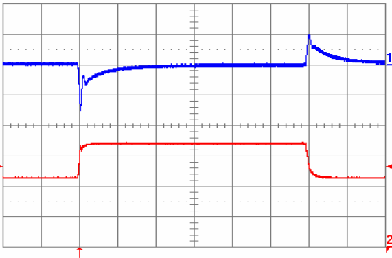
Fig. 3.3V.9: Output voltage response to load current step-change (22.5 A – 33.75 A – 22.5 A) at V_{in} = 48\text{ V} . Top trace: output voltage (100 mV/div.). Bottom trace: load current (10 A/div.). Current slew rate: 1 A/ \mu\text{s} . C_o = 470\text{ }\mu\text{F} tantalum + 1 \mu\text{F} ceramic. Time scale: 0.2 ms/div.
