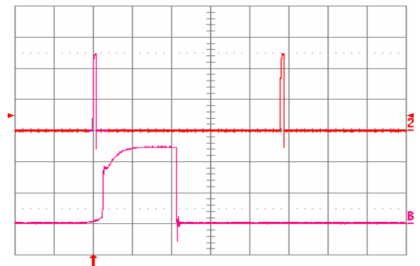
Fig. 2.5V.15: Load current (top trace, 20 A/div, 20 ms/div) into a 10\ \text{m}\Omega short circuit during restart, at V_{in} = 48\ \text{V} . Bottom trace (20 A/div, 1 ms/div) is an expansion of the on-time portion of the top trace.
