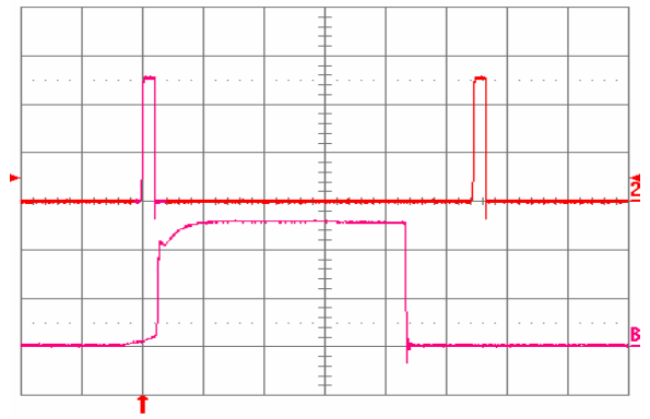
Fig. 1.5V.15: Load current (top trace, 20 A/div, 20 ms/div) into a 10 m \Omega short circuit during restart, at V_{in} = 48 V. Bottom trace (20 A/div, 1 ms/div) is an expansion of the on-time portion of the top trace.
