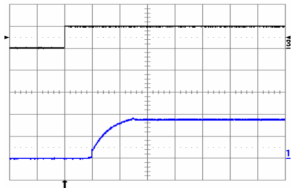
Fig. 1.8V.8: Turn-on transient at full rated load current (resistive) plus 40,000 \mu F at V_{in} = 48 V, triggered via ON/OFF pin. Top trace: ON/OFF signal (5 V/div.). Bottom trace: output voltage (1 V/div.). Time scale: 2 ms/div.
