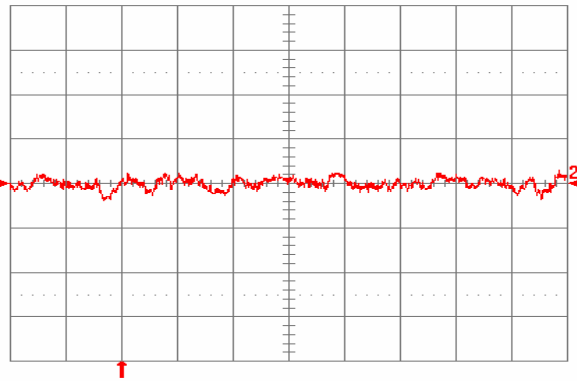
Fig. 1.5V.12: Input reflected ripple current, i_s (10 mA/div), measured through 10 \mu H at the source at full rated load current and V_{in} = 48 V. Refer to Fig. 1.5V.11 for test setup. Time scale: 1 \mu s/div.
