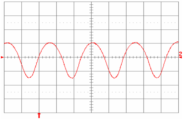
Fig. 1.5V.13: Input reflected ripple current, i_c (100 mA/div), measured at input terminals at full rated load current and V_{in} = 48 V. Refer to Fig. 1.5V.11 for test setup. Time scale: 1 \mu s/div.
