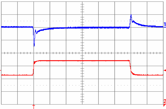
Fig. 2.0V.9: Output voltage response to load current step-change (22.5 A – 33.75 A – 22.5 A) at V_{in} = 48\text{ V} . Top trace: output voltage (100 mV/div.). Bottom trace: load current (10 A/div.). Current slew rate: 1 A/ \mu\text{s} . C_o = 470\text{ }\mu\text{F} tantalum + 1 \mu\text{F} ceramic. Time scale: 0.2 ms/div.
