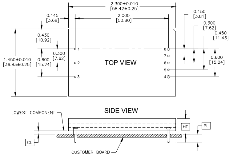
QM48T Pinout (Through-hole)
