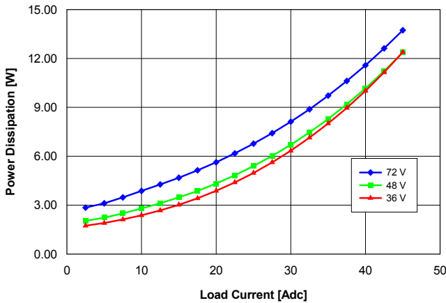
Fig. 1.8V.5: Power dissipation vs. load current and input voltage for converter mounted vertically with air flowing from pin 3 to pin 1 at a rate of 300 LFM (1.5 m/s) and T_a = 25^\circ\text{C} .
