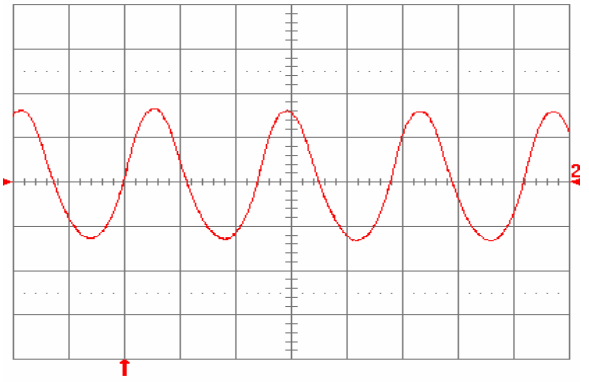
Fig. 3.3V.13: Input reflected ripple current, i_c (100 mA/div), measured at input terminals at full rated load current and V_{in} = 48 V. Refer to Fig. 3.3V.11 for test setup. Time scale: 1 µs/div.
