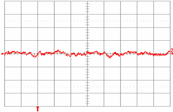
Fig. 2.5V.12: Input reflected ripple current, i_s (10 mA/div), measured through 10\ \mu\text{H} at the source at full rated load current and V_{in} = 48\ \text{V} . Refer to Fig. 2.5V.11 for test setup. Time scale: 1\ \mu\text{s}/\text{div} .
