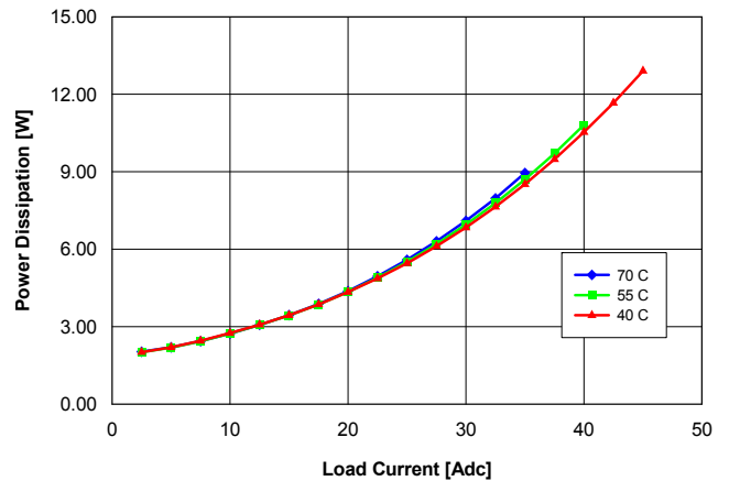
Fig. 1.8V.6: Power dissipation vs. load current and ambient temperature for converter mounted vertically with V_{in} = 48\text{ V} and air flowing from pin 3 to pin 1 at a rate of 200 LFM (1.0 m/s).
