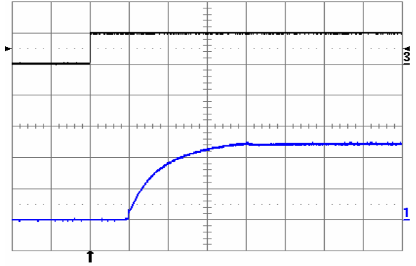
Fig. 2.5V.8: Turn-on transient at full rated load current (resistive) plus 40,000 \mu\text{F} at V_{in} = 48\text{ V} , triggered via ON/OFF pin. Top trace: ON/OFF signal (5 V/div.). Bottom trace: output voltage (1 V/div.). Time scale: 2 ms/div.
