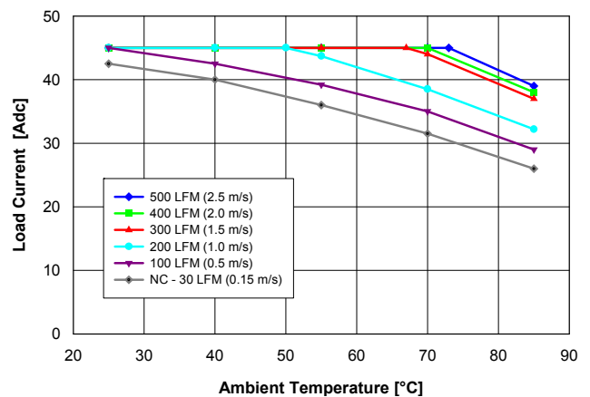
Fig. 1.8V.2: Available load current vs. ambient air temperature and airflow rates for QM48T45018 converter with B height pins mounted horizontally with V_{in} = 48\text{ V} , air flowing from pin 3 to pin 1, and MOSFET temperature \leq 120^\circ\text{C} .
