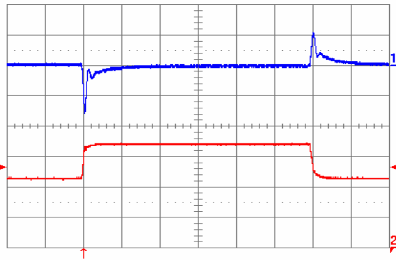
Fig. 1.2V.9: Output voltage response to load current step-change (22.5 A – 33.75 A – 22.5 A) at V_{in} = 48 V. Top trace: output voltage (100 mV/div.). Bottom trace: load current (10 A/div.). Current slew rate: 1 A/ \mu s. C_o = 470 \mu F tantalum + 1 \mu F ceramic. Time scale: 0.2 ms/div.
