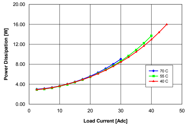
Fig. 2.5V.6: Power dissipation vs. load current and ambient temperature for converter mounted vertically with V_{in} = 48\text{ V} and air flowing from pin 3 to pin 1 at a rate of 200 LFM (1.0 m/s).
