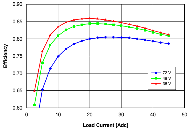
Fig. 1.0V.3: Efficiency vs. load current and input voltage for converter mounted vertically with air flowing from pin 3 to pin 1 at a rate of 300 LFM (1.5 m/s) and T_a = 25^\circ\text{C} .
