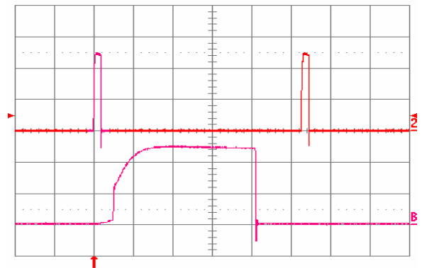
Fig. 1.8V.15: Load current (top trace, 20 A/div, 20 ms/div) into a 10 m \Omega short circuit during restart, at V_{in} = 48 V. Bottom trace (20 A/div, 1 ms/div) is an expansion of the on-time portion of the top trace.
