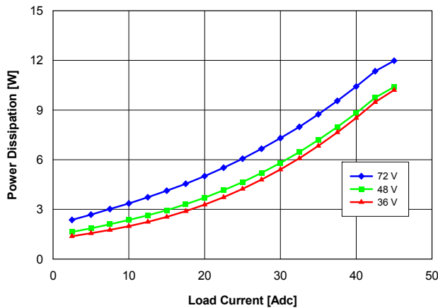
Fig. 1.0V.5: Power dissipation vs. load current and input voltage for converter mounted vertically with air flowing from pin 3 to pin 1 at a rate of 300 LFM (1.5 m/s) and T_a = 25^\circ\text{C} .
