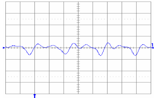
Fig. 1.0V.10: Output voltage ripple (20 mV/div.) at full rated load current into a resistive load with C_o = 10 \mu F tantalum + 1 \mu F ceramic and V_{in} = 48 V. Time scale: 1 \mu s/div.
