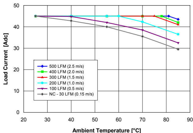
Fig. 1.0V.2: Available load current vs. ambient air temperature and airflow rates for QM48T45010 converter with B height pins mounted horizontally with V_{in} = 48\text{ V} , air flowing from pin 3 to pin 1, and MOSFET temperature \leq 120^\circ\text{C} .
