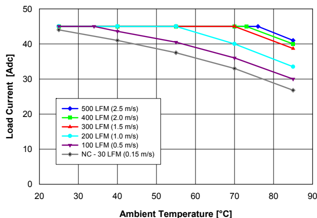
Fig. 1.5V.2: Available load current vs. ambient air temperature and airflow rates for QM48T45015 converter with B height pins mounted horizontally with V_{in} = 48\text{ V} , air flowing from pin 3 to pin 1, and MOSFET temperature \leq 120^\circ\text{C} .
