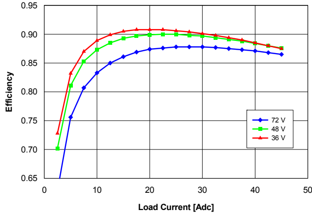
Fig. 2.0V.3: Efficiency vs. load current and input voltage for converter mounted vertically with air flowing from pin 3 to pin 1 at a rate of 300 LFM (1.5 m/s) and T_a = 25^\circ\text{C} .
