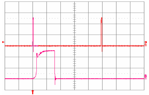
Fig. 3.3V.15: Load current (top trace, 20 A/div, 20 ms/div) into a 10 mΩ short circuit during restart, at V_{in} = 48 V. Bottom trace (20 A/div, 1 ms/div) is an expansion of the on-time portion of the top trace.
