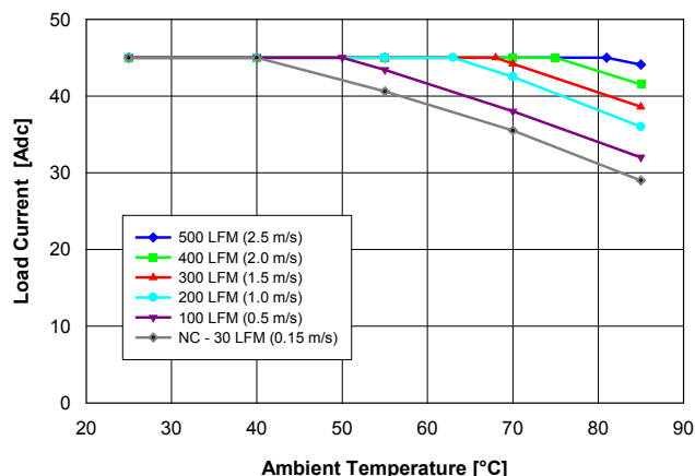
Fig. 1.0V.1: Available load current vs. ambient air temperature and airflow rates for QM48T45010 converter with B height pins mounted vertically with V_{in} = 48\text{ V} , air flowing from pin 3 to pin 1, and MOSFET temperature \leq 120^\circ\text{C} .
