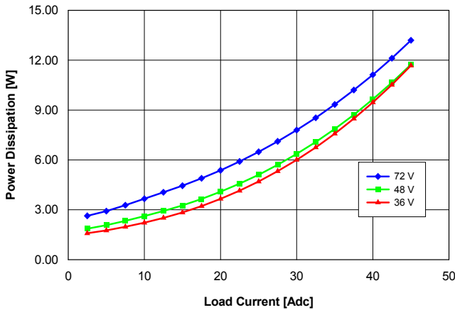
Fig. 1.5V.5: Power dissipation vs. load current and input voltage for converter mounted vertically with air flowing from pin 3 to pin 1 at a rate of 300 LFM (1.5 m/s) and T_a = 25^\circ\text{C} .
