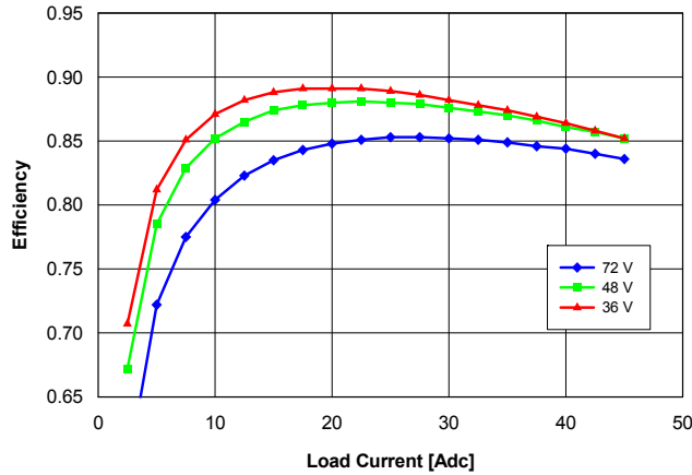
Fig. 1.5V.3: Efficiency vs. load current and input voltage for converter mounted vertically with air flowing from pin 3 to pin 1 at a rate of 300 LFM (1.5 m/s) and T_a = 25^\circ\text{C} .
