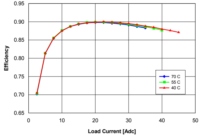
Fig. 2.0V.4: Efficiency vs. load current and ambient temperature for converter mounted vertically with V_{in} = 48\text{ V} and air flowing from pin 3 to pin 1 at a rate of 200 LFM (1.0 m/s).
