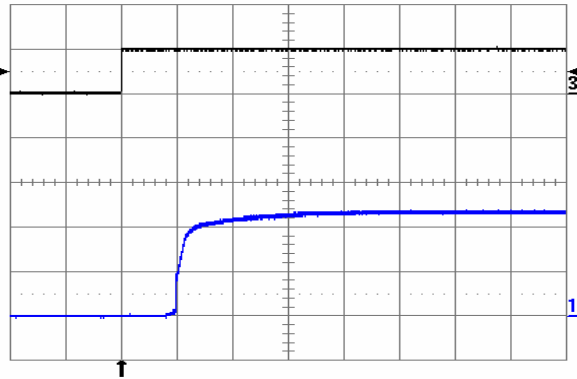
Fig. 1.2V.7: Turn-on transient at full rated load current (resistive) with no output capacitor at V_{in} = 48 V, triggered via ON/OFF pin. Top trace: ON/OFF signal (5 V/div.). Bottom trace: output voltage (1 V/div.). Time scale: 2 ms/div.
