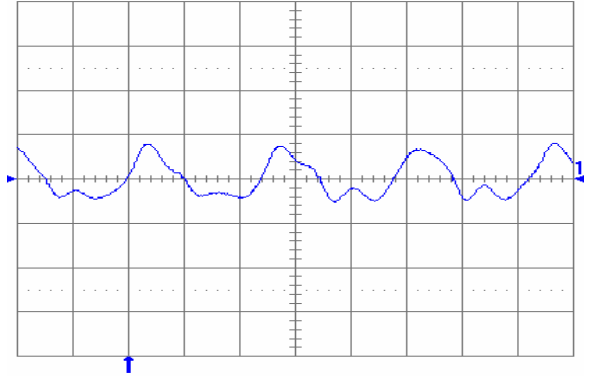
Fig. 3.3V.10: Output voltage ripple (20 mV/div.) at full rated load current into a resistive load with C_o = 10\text{ }\mu\text{F} tantalum + 1 \mu\text{F} ceramic and V_{in} = 48\text{ V} . Time scale: 1 \mu\text{s} /div.
