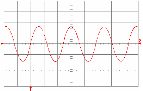
Fig. 2.5V.13: Input reflected ripple current, i_c (100 mA/div), measured at input terminals at full rated load current and V_{in} = 48\ \text{V} . Refer to Fig. 2.5V.11 for test setup. Time scale: 1\ \mu\text{s}/\text{div} .
