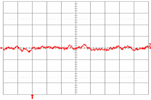
Fig. 2.0V.12: Input reflected ripple current, i_s (10 mA/div), measured through 10 \mu H at the source at full rated load current and V_{in} = 48 V. Refer to Fig. 2.0V.11 for test setup. Time scale: 1 \mu s/div.
