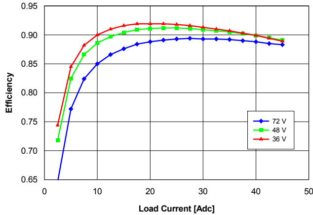
Fig. 2.5V.3: Efficiency vs. load current and input voltage for converter mounted vertically with air flowing from pin 3 to pin 1 at a rate of 300 LFM (1.5 m/s) and T_a = 25^\circ\text{C} .
