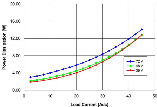
Fig. 2.0V.5: Power dissipation vs. load current and input voltage for converter mounted vertically with air flowing from pin 3 to pin 1 at a rate of 300 LFM (1.5 m/s) and T_a = 25^\circ\text{C} .
