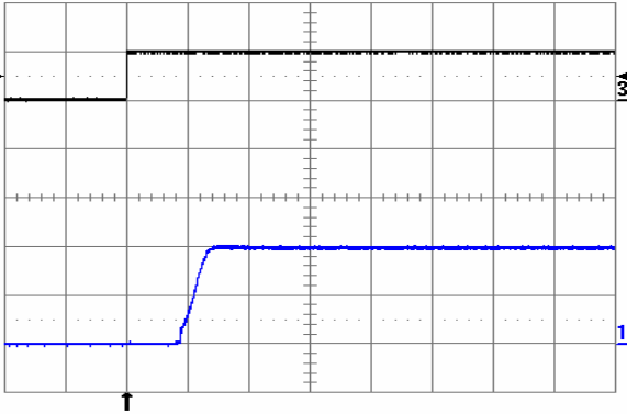
Fig. 2.0V.7: Turn-on transient at full rated load current (resistive) with no output capacitor at V_{in} = 48\text{ V} , triggered via ON/OFF pin. Top trace: ON/OFF signal (5 V/div.). Bottom trace: output voltage (1 V/div.). Time scale: 2 ms/div.
