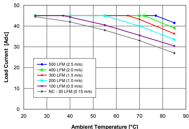
Fig. 1.5V.1: Available load current vs. ambient air temperature and airflow rates for QM48T45015 converter with B height pins mounted vertically with V_{in} = 48\text{ V} , air flowing from pin 3 to pin 1, and MOSFET temperature \leq 120^\circ\text{C} .
