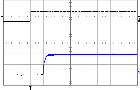
Fig. 1.0V.7: Turn-on transient at full rated load current (resistive) with no output capacitor at V_{in} = 48 V, triggered via ON/OFF pin. Top trace: ON/OFF signal (5 V/div.). Bottom trace: output voltage (1V/div.). Time scale: 2 ms/div.
