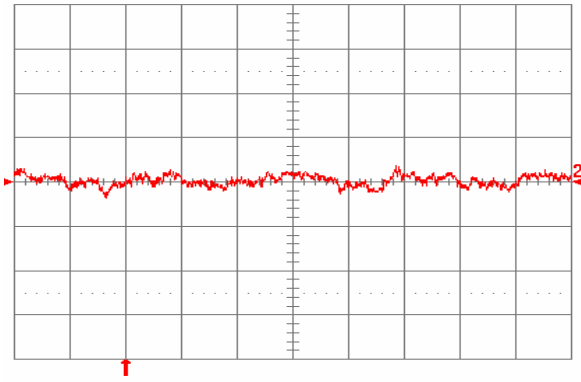
Fig. 3.3V.12: Input reflected ripple current, i_s (10 mA/div), measured through 10 µH at the source at full rated load current and V_{in} = 48 V. Refer to Fig. 3.3V.11 for test setup. Time scale: 1 µs/div.
