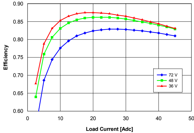
Fig. 1.2V.3: Efficiency vs. load current and input voltage for converter mounted vertically with air flowing from pin 3 to pin 1 at a rate of 300 LFM (1.5 m/s) and T_a = 25^\circ\text{C} .
