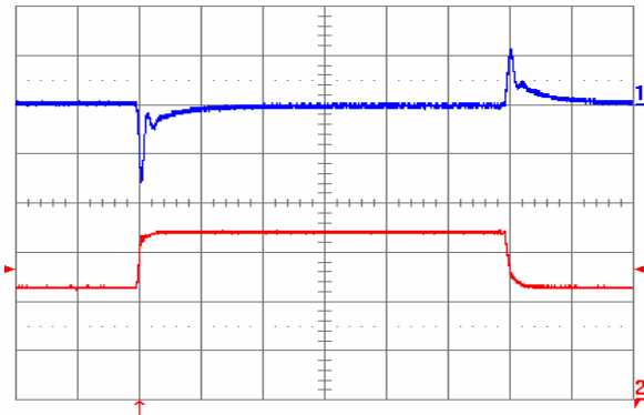
Fig. 1.0V.9: Output voltage response to load current step-change (22.5 A – 33.75 A – 22.5 A) at V_{in} = 48 V. Top trace: output voltage (100 mV/div.). Bottom trace: load current (10 A/div.). Current slew rate: 1 A/ \mu s. C_o = 470 \mu F tantalum + 1 \mu F ceramic. Time scale: 0.2 ms/div.
