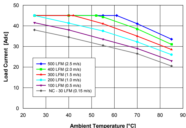
Fig. 3.3V.1: Available load current vs. ambient air temperature and airflow rates for QM48T45033 converter with B height pins mounted vertically with V_{in} = 48\text{ V} , air flowing from pin 3 to pin 1, and MOSFET temperature \leq 120^\circ\text{C} .
