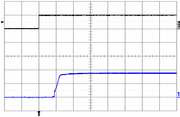
Fig. 1.8V.7: Turn-on transient at full rated load current (resistive) with no output capacitor at V_{in} = 48 V, triggered via ON/OFF pin. Top trace: ON/OFF signal (5 V/div.). Bottom trace: output voltage (1 V/div.). Time scale: 2 ms/div.
