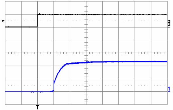
Fig. 1.2V.8: Turn-on transient at full rated load current (resistive) plus 40,000 \mu F at V_{in} = 48 V, triggered via ON/OFF pin. Top trace: ON/OFF signal (5 V/div.). Bottom trace: output voltage (1 V/div.). Time scale: 2 ms/div.
