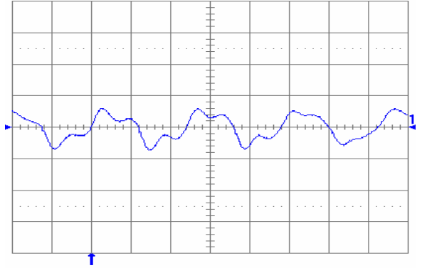
Fig. 2.5V.10: Output voltage ripple (20 mV/div.) at full rated load current into a resistive load with C_o = 10\text{ }\mu\text{F} tantalum + 1 \mu\text{F} ceramic and V_{in} = 48\text{ V} . Time scale: 1 \mu\text{s} /div.
