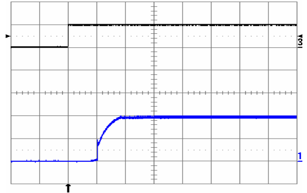
Fig. 1.0V.8: Turn-on transient at full rated load current (resistive) plus 40,000 \mu F at V_{in} = 48 V, triggered via ON/OFF pin. Top trace: ON/OFF signal (5 V/div.). Bottom trace: output voltage (1 V/div.). Time scale: 2 ms/div.
