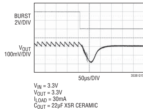
Transition From Burst Mode Operation to Fixed Frequency
