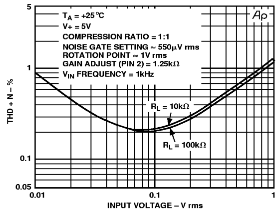
Figure 7. THD+N (%) vs. Input (V rms)
