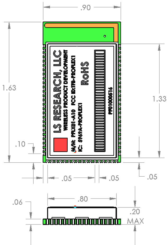
Figure 15 Basic dimensions
