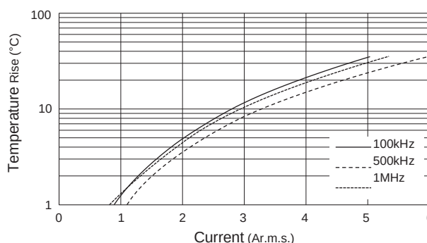
Ripple Current
