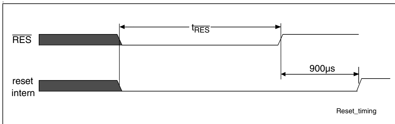
Figure 30 Reset Timing
