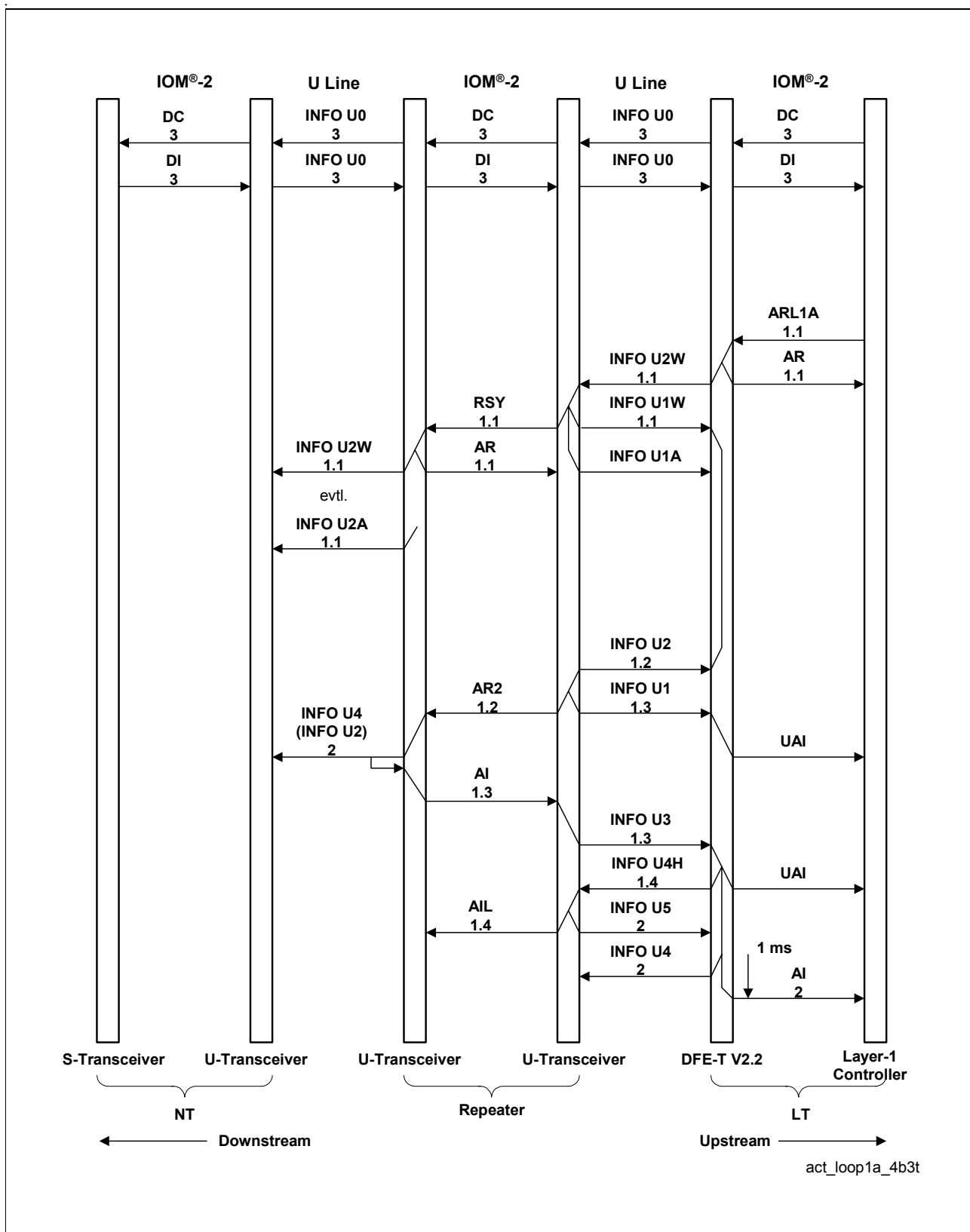
Figure 24 Activation of Loop#1A (Repeater)
