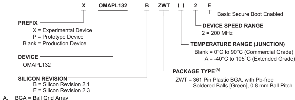
Figure 7-1. Device Nomenclature
