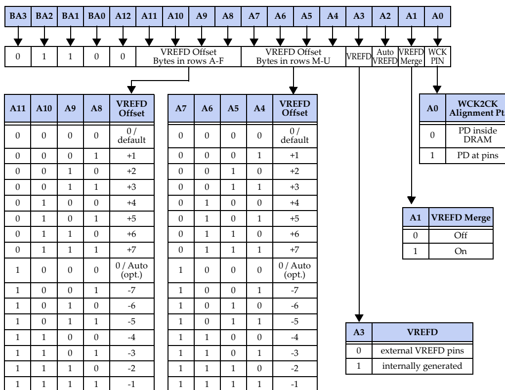
Figure 30. Mode Register 6 (MR6) Definition
