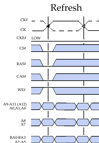
Figure 70. REFRESH command
