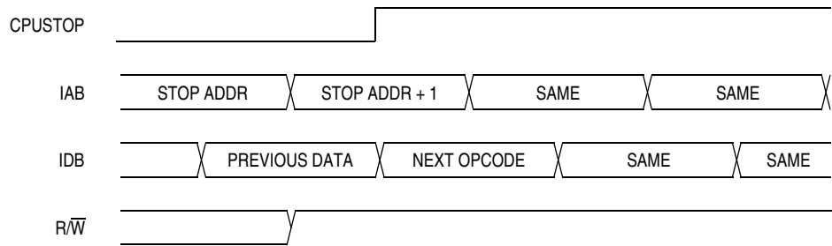
Figure 14-14. Stop Mode Entry Timing
