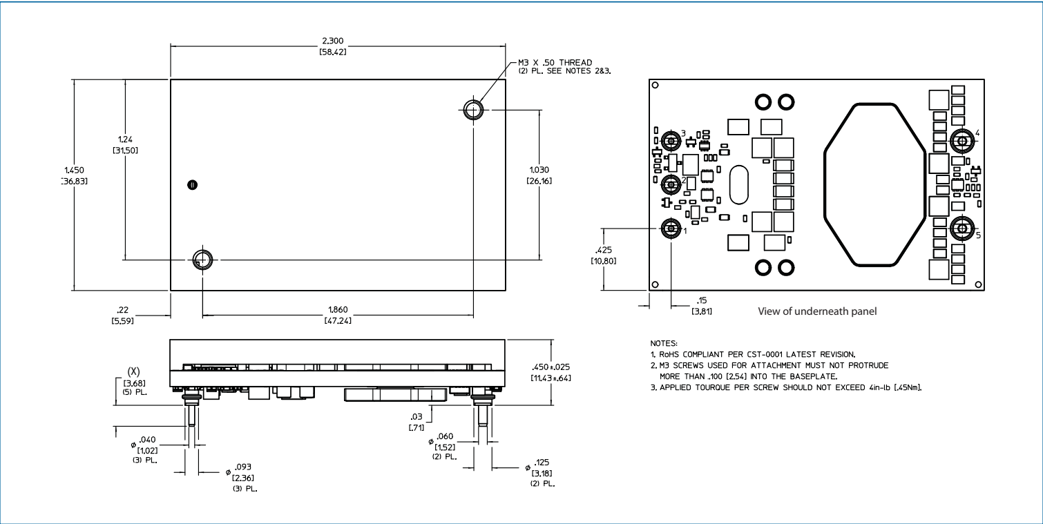
Figure 31 — IBC outline drawing - baseplate option
