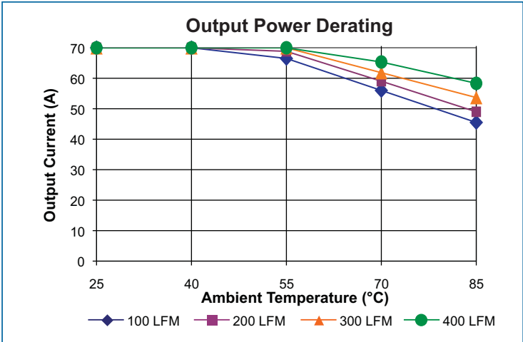
Figure 20 — Maximum output power derating vs ambient air temperature. Longitudinal airflow, Board and junction temperatures <125° C. Tested with IBC evaluation board IB054Q096T70N1-CB
