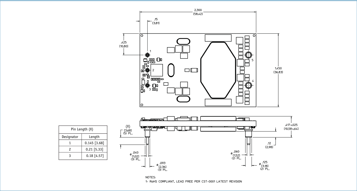
Figure 32 — IBC Outline drawing
