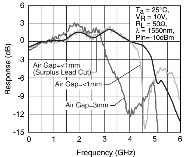
Fig. 4 Frequency Response
