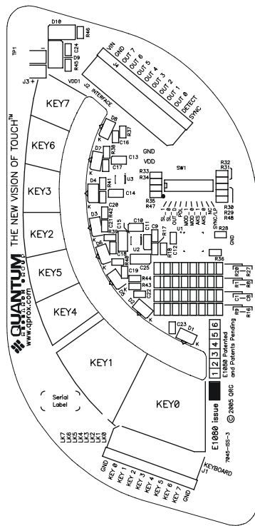
Figure 5 — Silkscreen Layer
