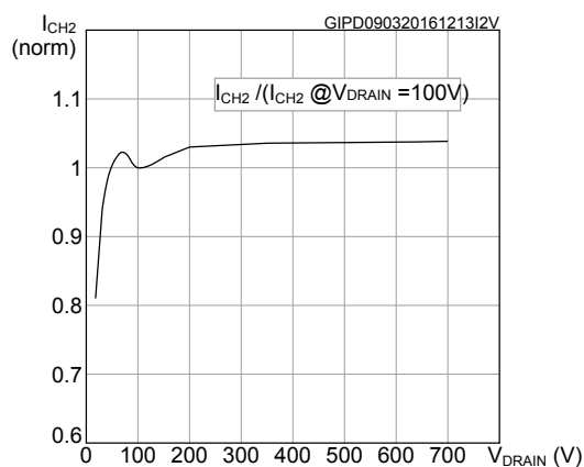
Figure 13. I_{CH2} vs V_{DRAIN}
