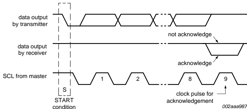
Fig 8. Acknowledgement on the I 2 C-bus
