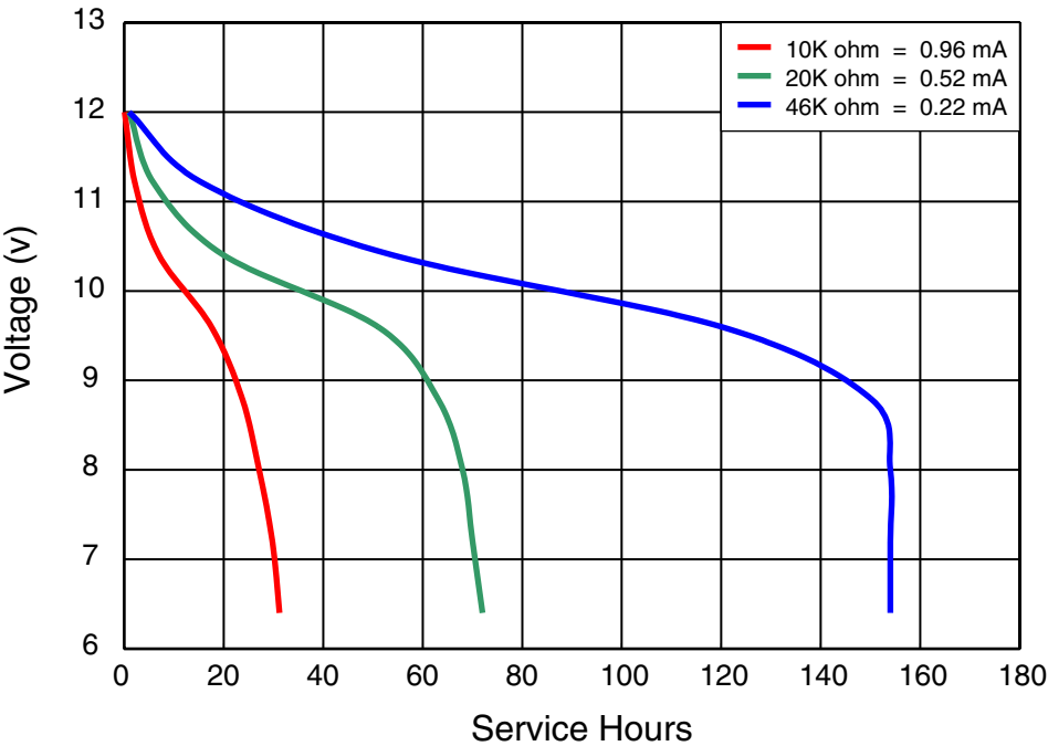
TYPICAL DISCHARGE CHARACTERISTICS AT 21°C (70°F)
