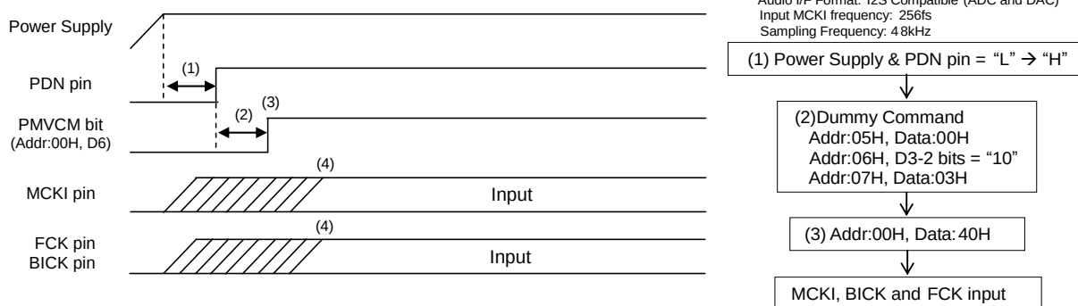
Figure 68. Clock Set Up Sequence (3)
