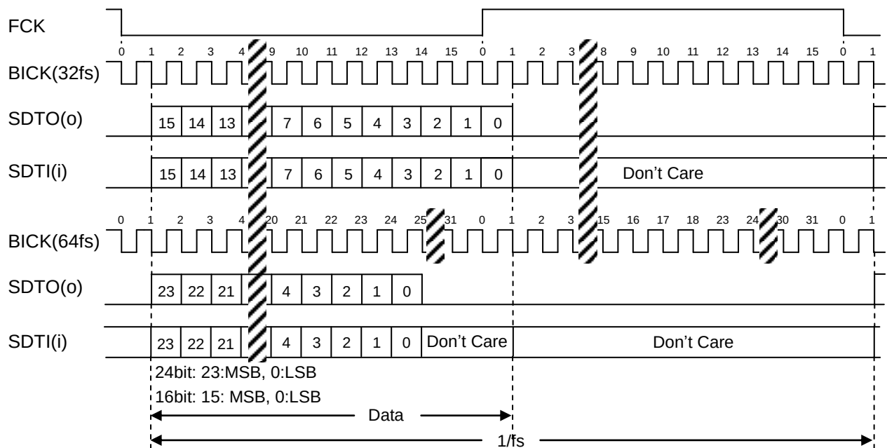
Figure 33. Mode 3 Timing
