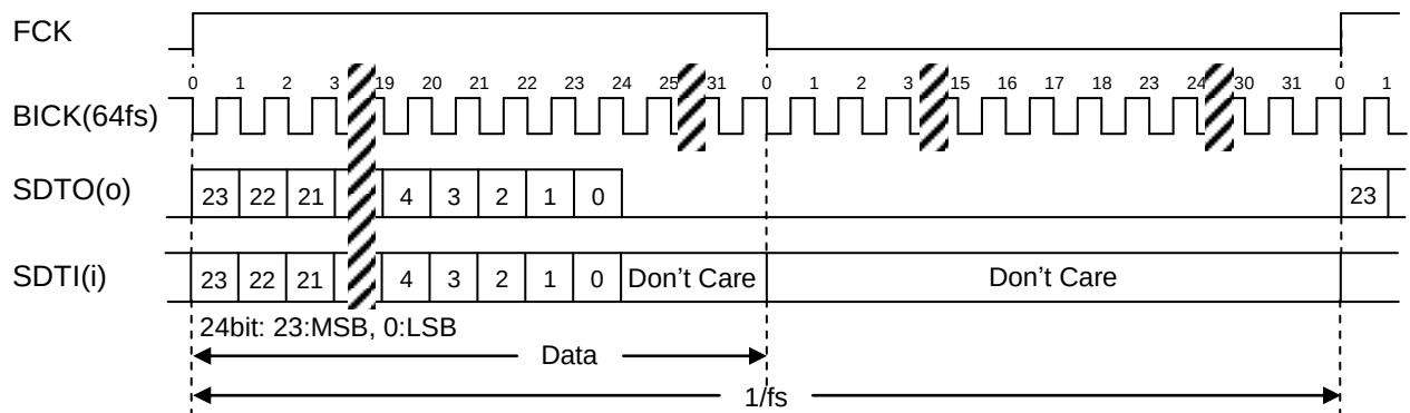
Figure 32. Mode 2 Timing
