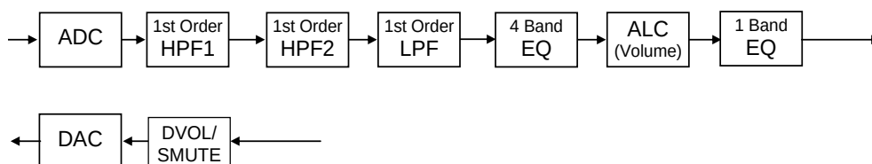
Figure 40. The Path in Recording Mode 1 &amp; Playback Mode 2 (default)
