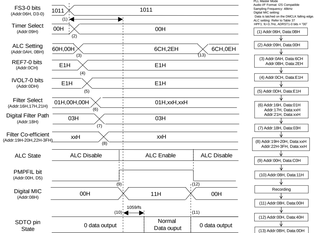
Figure 71. Digital Microphone Input Recording Sequence
