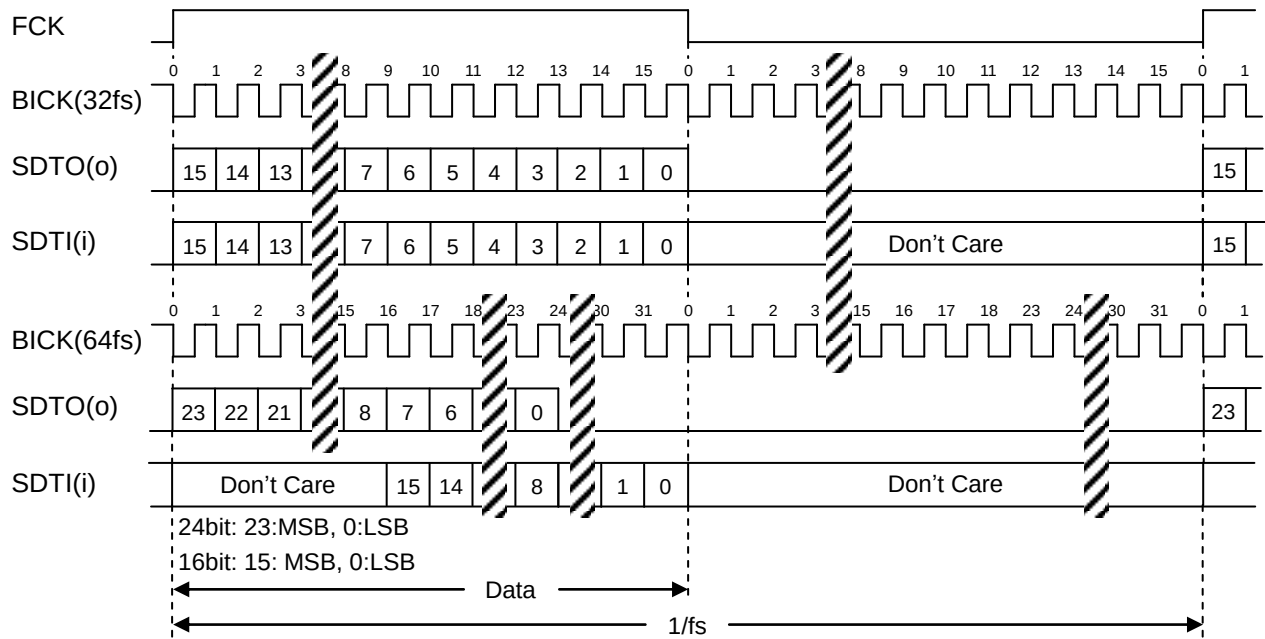
Figure 31. Mode 1 Timing
