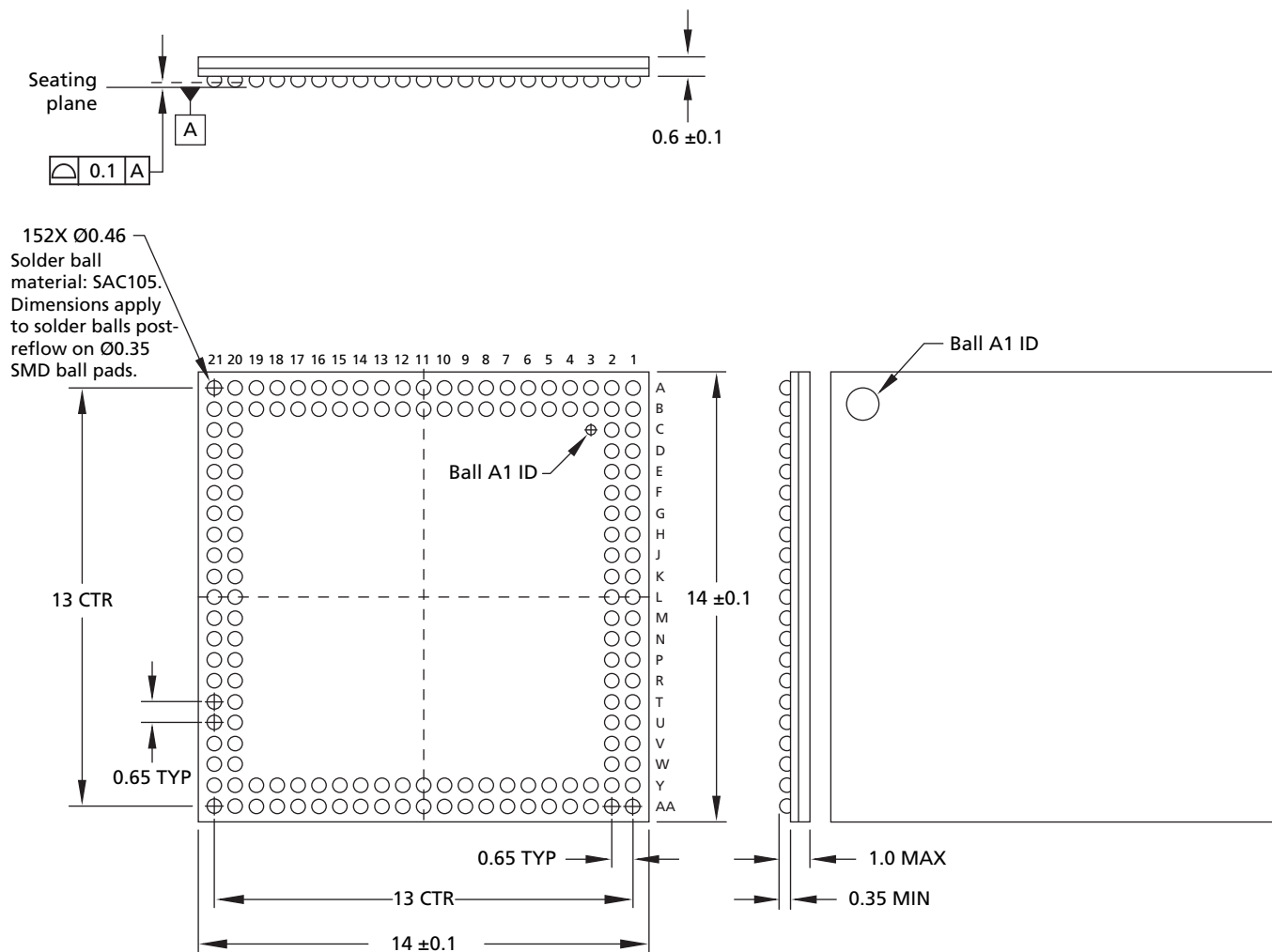
Figure 6: 152-Ball VFBGA Package, 1.0mm (Package Code: CG)
