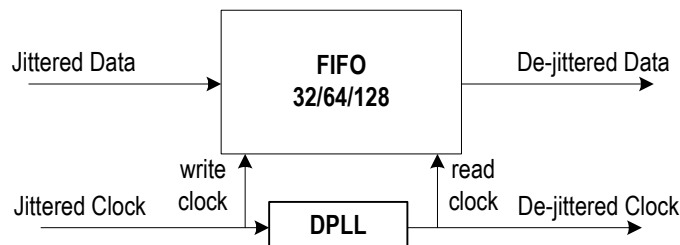
Figure-19 Jitter Attenuator
