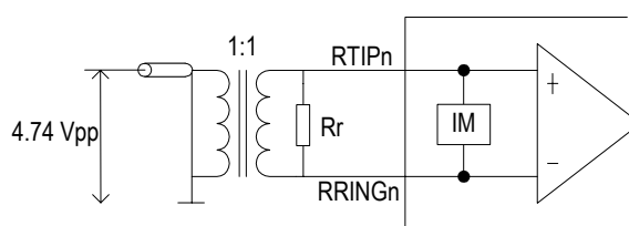
Figure-5 Receive Differential Line Interface with Coaxial Cable (with transformer)
