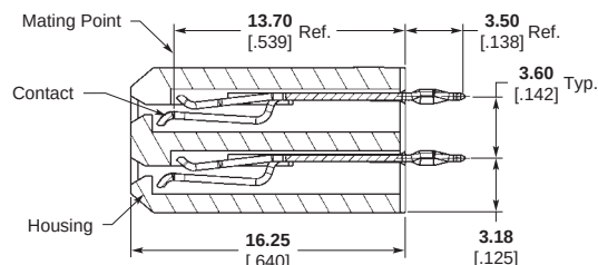
Section Y-Y
