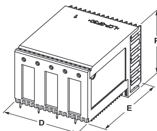
Plug (Daughtercard)
