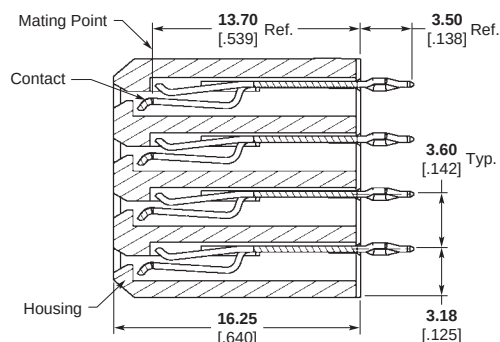
Section Y-Y
