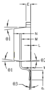
SIDE VIEW 1
