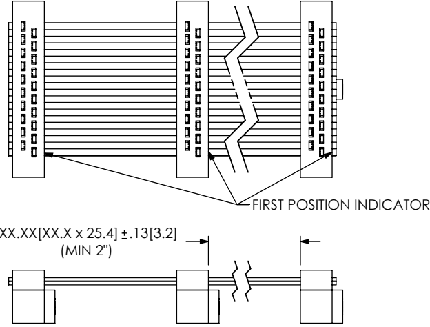
FIG 7 (FFSD-10-D-XX.XX-01-X-N-DXX SHOWN) (SAME AS FIG 1, DIFFERENT AS SHOWN) (2.00[50.8] MINIMUM, 1.00[25.4] INCREMENTS)
