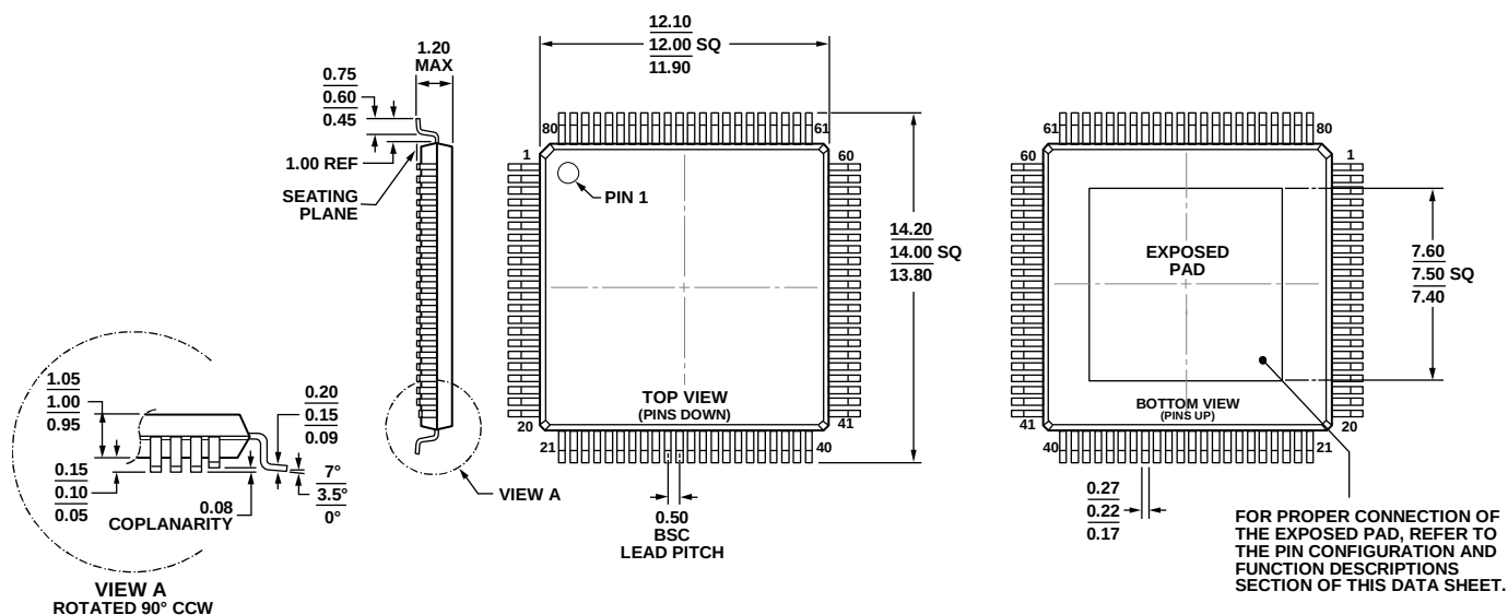
Figure 7. 80-Lead Thin Quad Flat Package, Exposed Pad [TQFP_EP]
