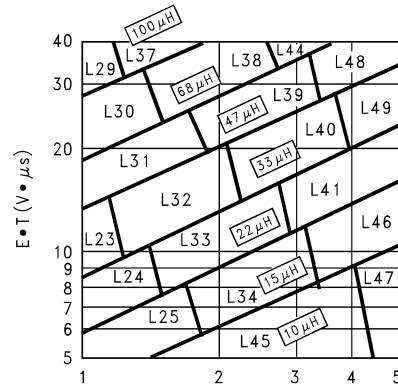
Figure 17. LM2679-Adjustable Voltage
