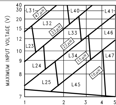
Figure 15. LM2679-5 V
