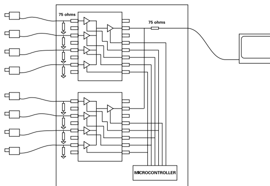
Fig.1: Typical Application for 8 channel CCTV
