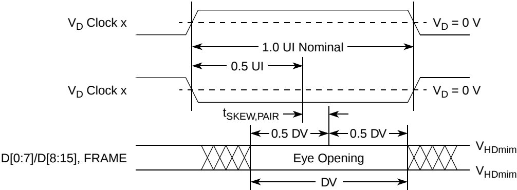
Figure 42. Data to Clock Skew
