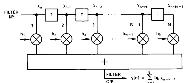
Figure 17. Transversal Filter
