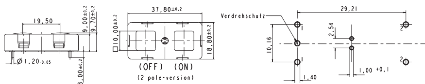
PCB footprint
