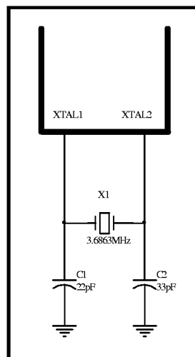
Figure 1: Crystal Connection
