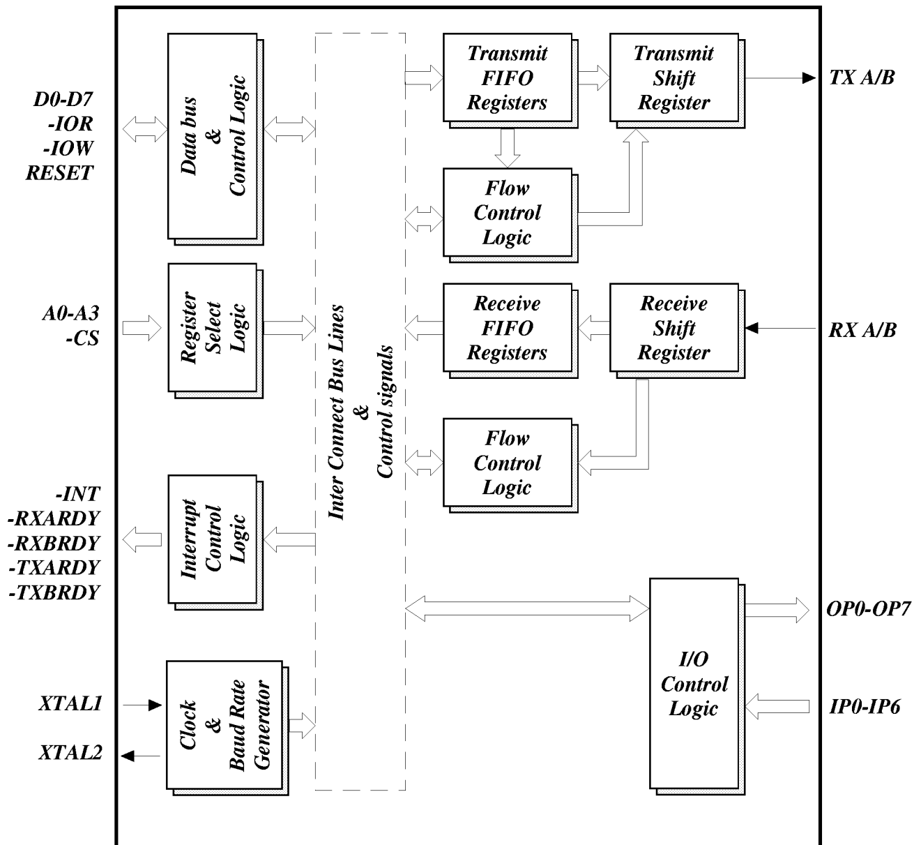
Block Diagram
