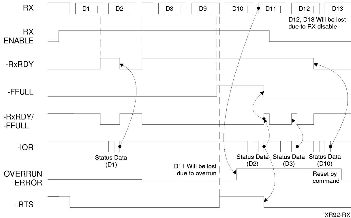
Figure 5: Receive Timing
