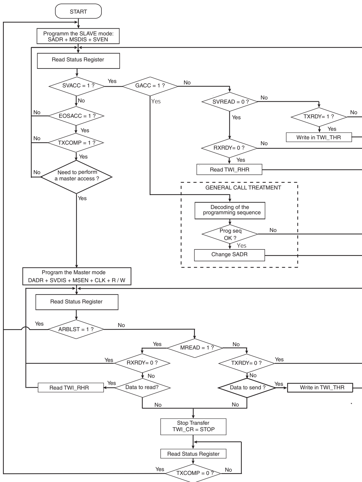
Figure 28-23. Multi-master Flowchart
