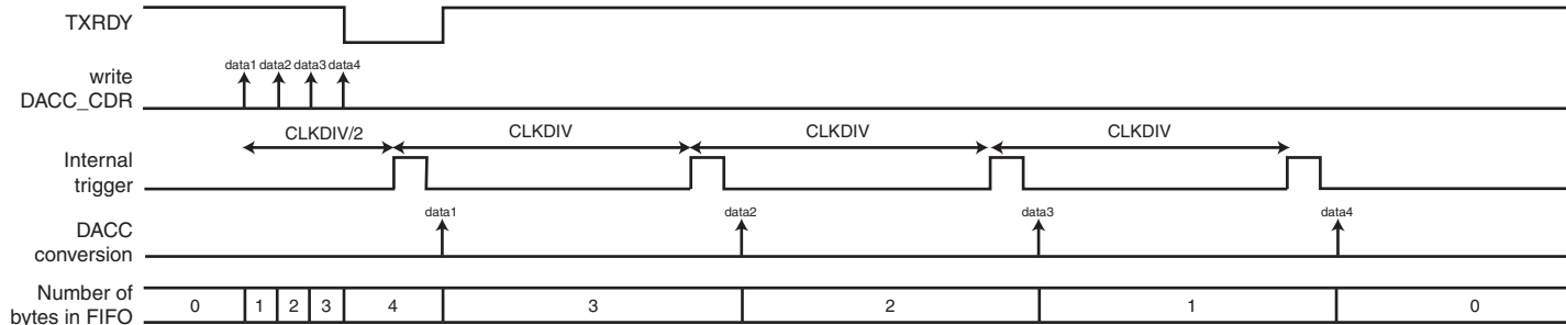
Figure 34-2. Internal trigger
