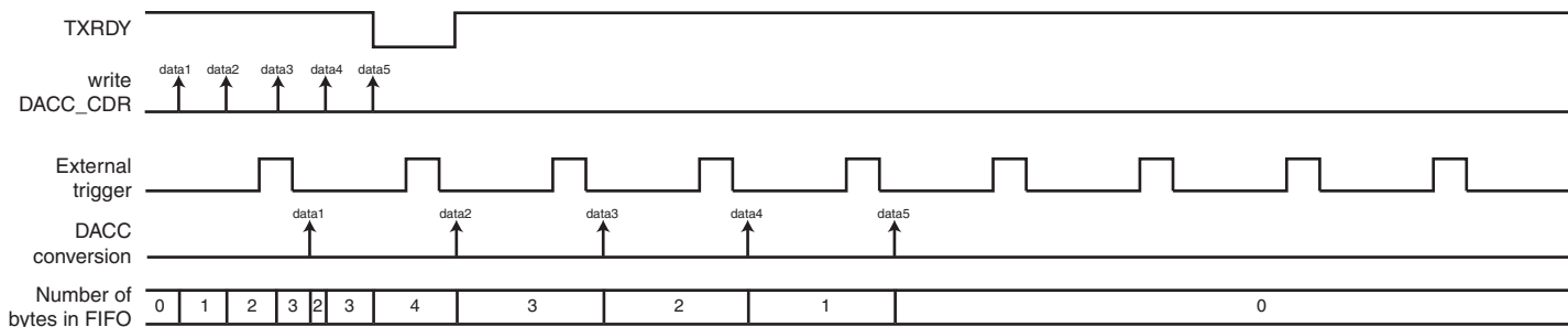
Figure 34-3. External trigger
