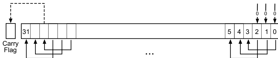
Figure 10-6. LSL #3
