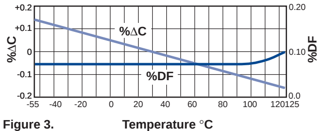
Figure 3. Temperature °C Capacitance & DF vs Temperature - C0G
