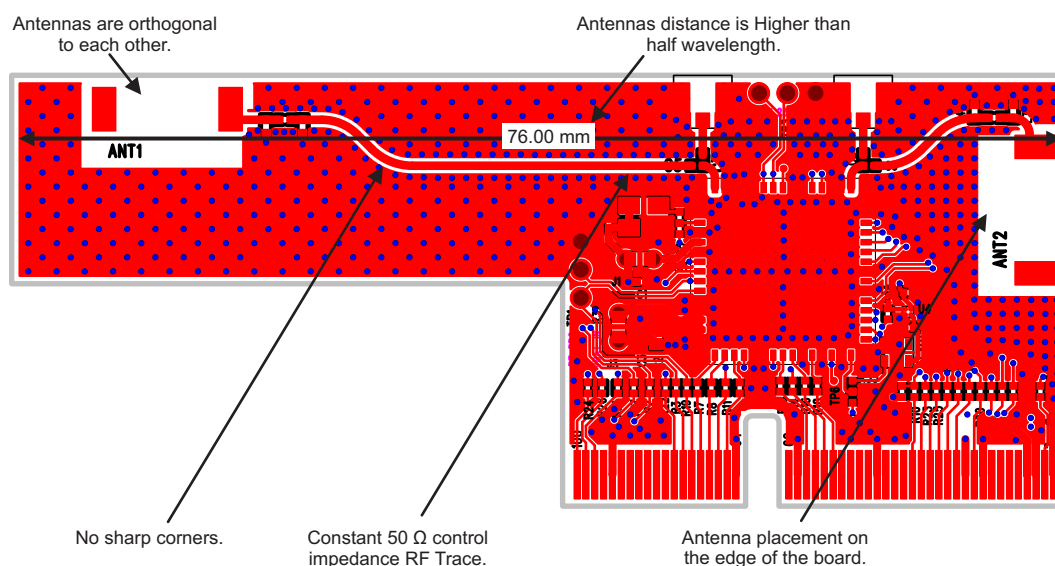
Figure 7-2. Location of Antenna and RF Trace Routing on the WL1837MODCOM8I Board
