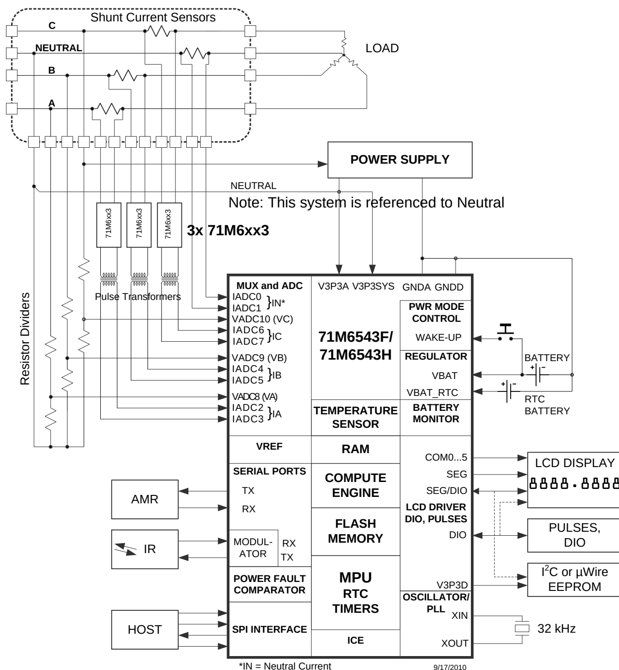
Figure 4: Current Sensors Connected to the 71M6543F/H or 71M6545/H with Three 71M6xx3
