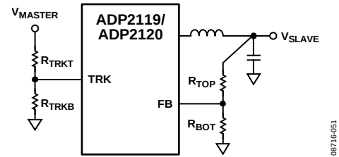
Figure 51. Voltage Tracking
