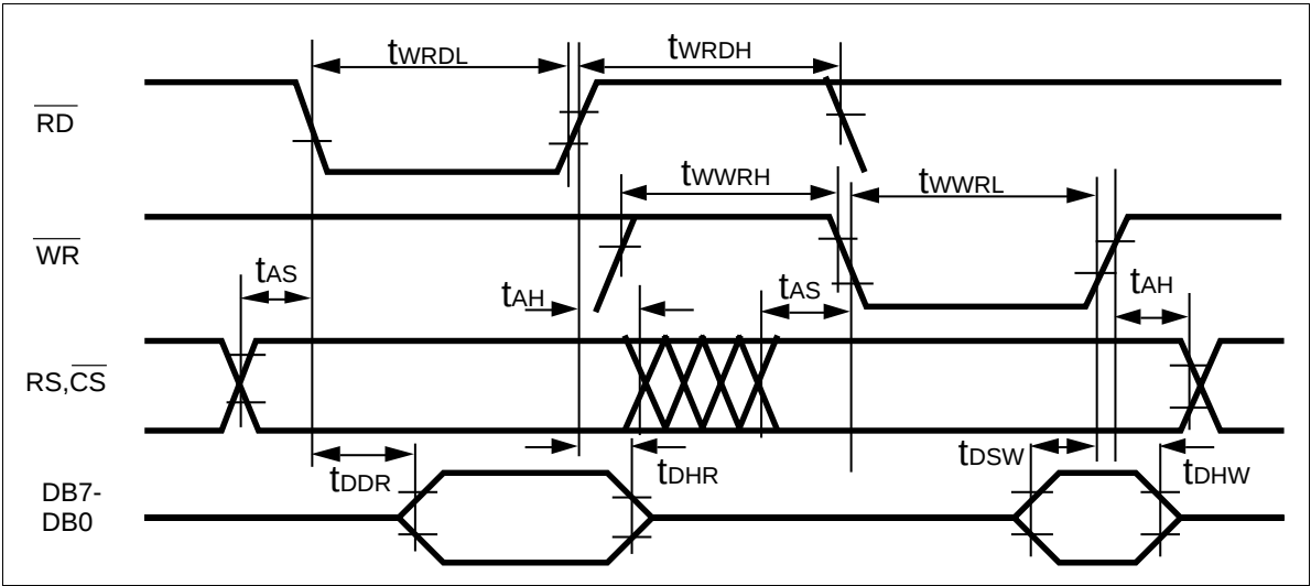
Figure 49 MPU Interface
