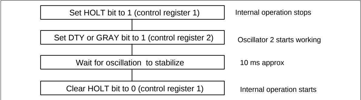
Figure 39 Procedure for Changing Oscillator
