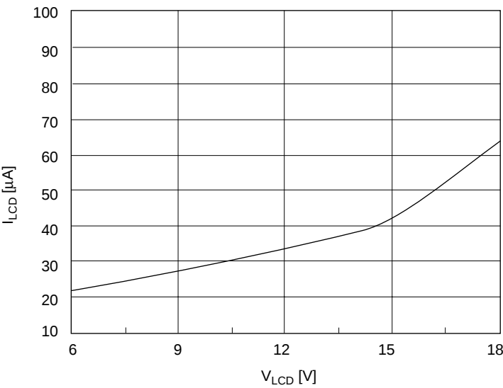
Figure 53 ILCD (VCC = 3 V)
