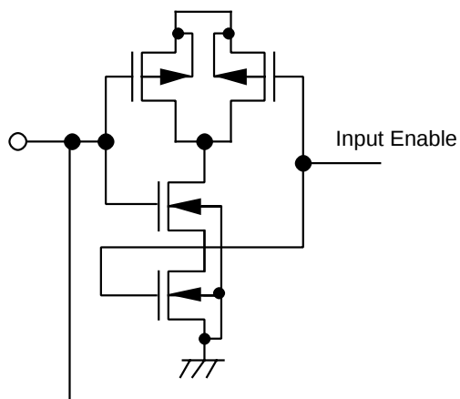
Figure 47 Terminal Configuration
