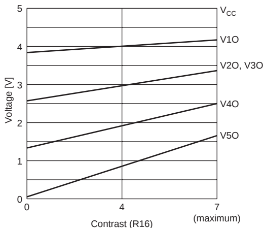
Example.2 LCD bias level
