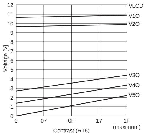
Example.1 LCD bias level
