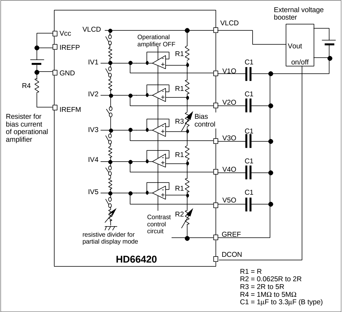
Figure 42 Power Supply Circuit
