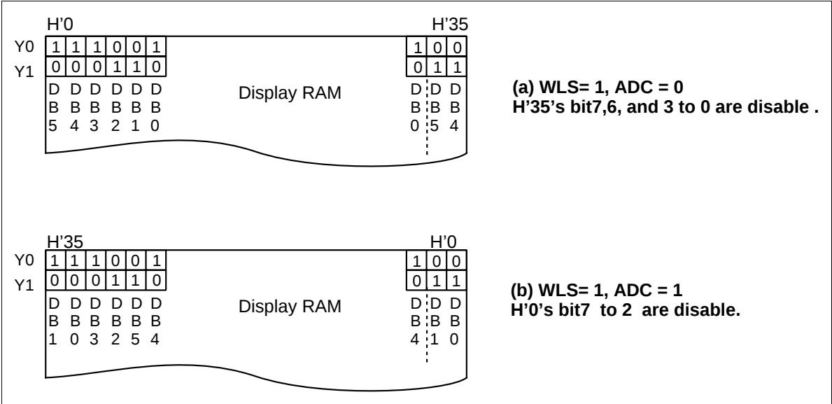
Figure 25 Display RAM Bits Map
