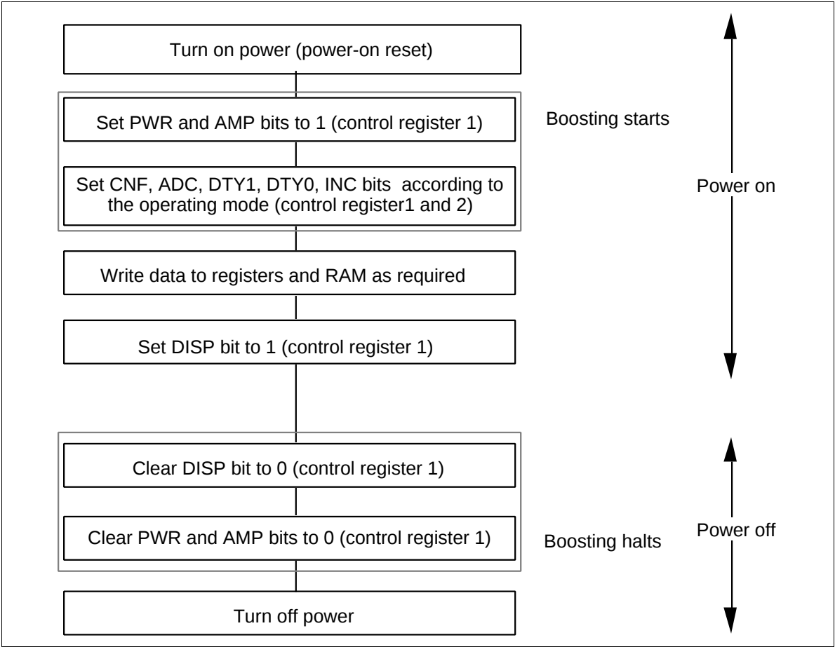
Figure 40 Procedure for Turning Power Supply On/Off
