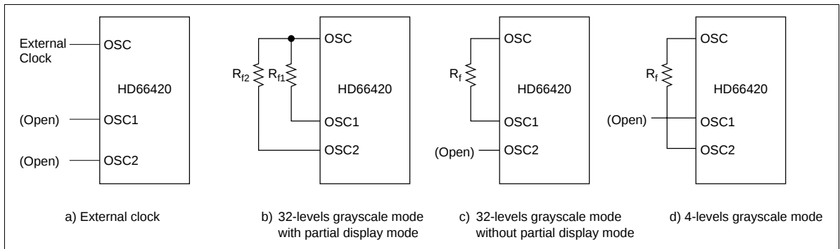
Figure 41 Oscillator Connections
