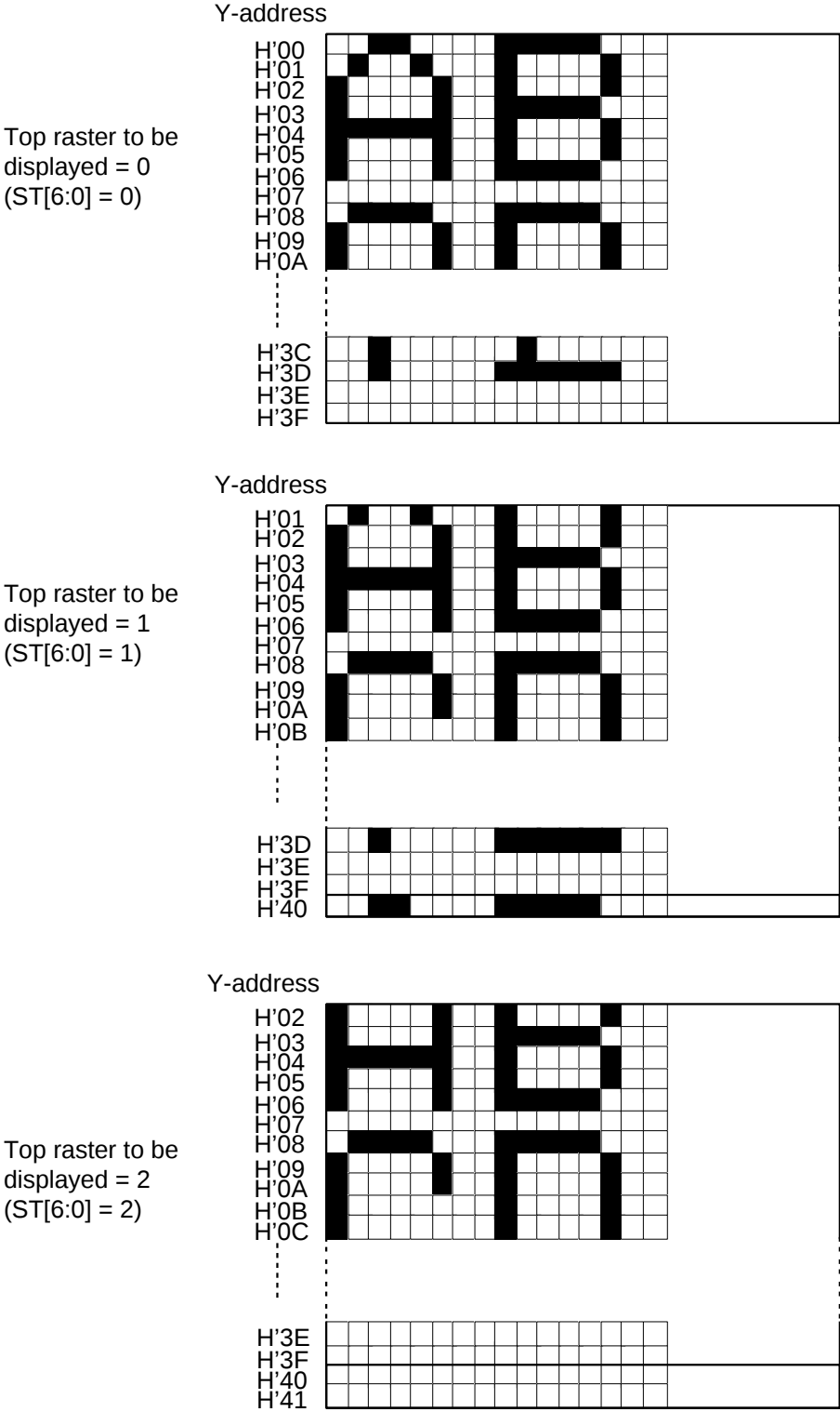
Figure 34 Vertical Scroll : 1/64Duty Cycle
