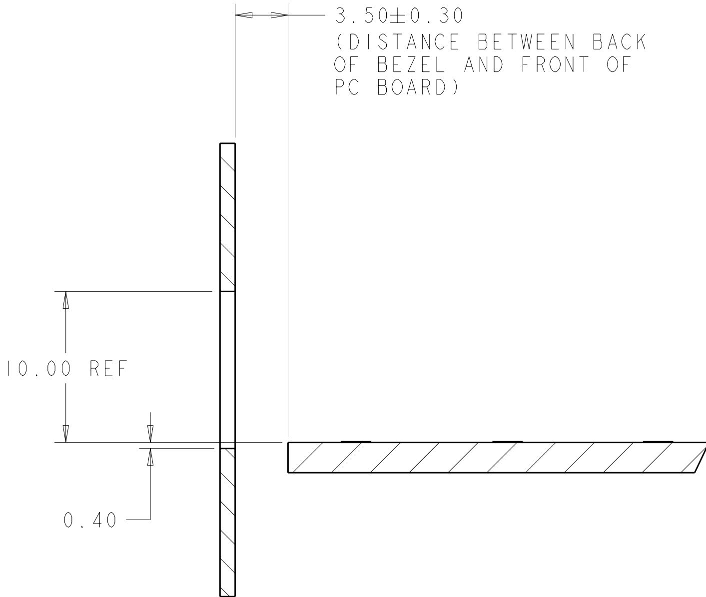
SECTION X-X
