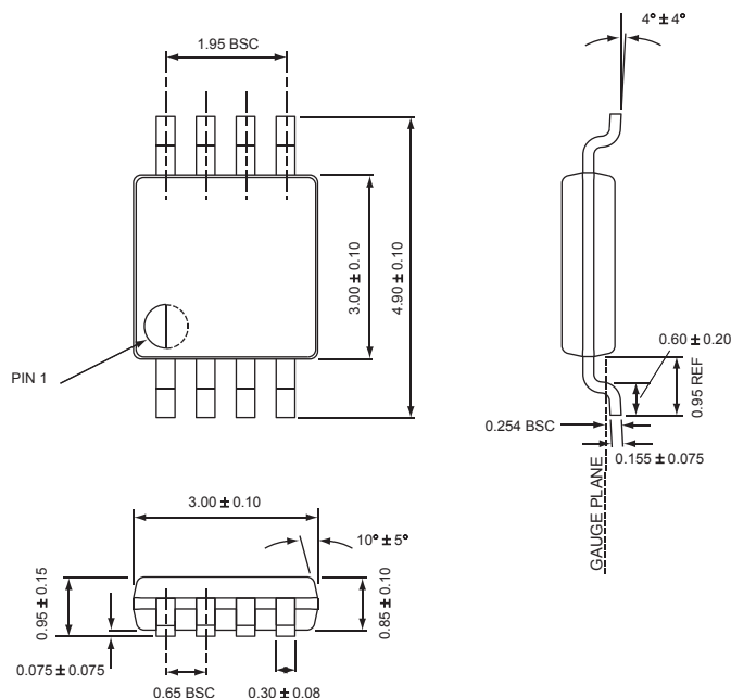
MSOP-8
