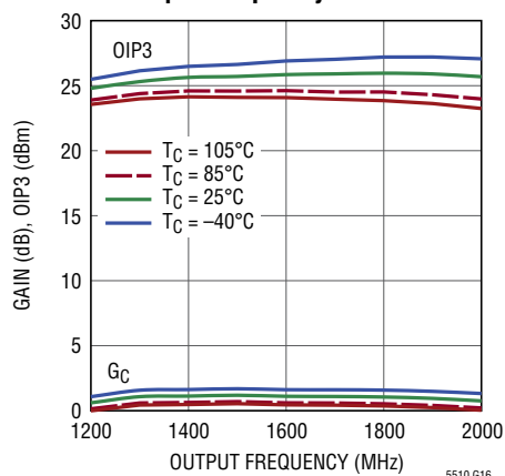
Conversion Gain and OIP3 vs Output Frequency
