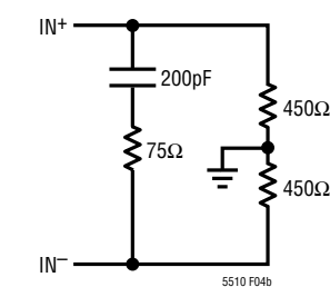
Figure 4b. IN Port Equivalent Circuit (< 1GHz)
