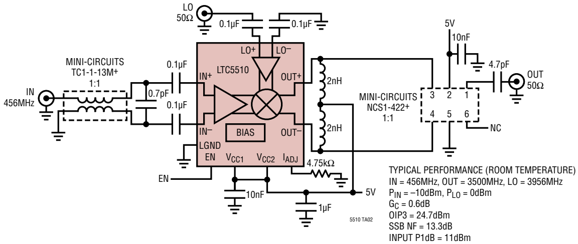
Upmixer with 3.3GHz to 3.8GHz Output
