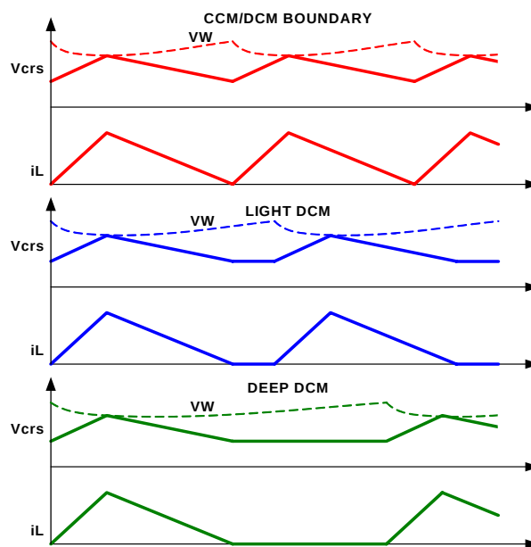
FIGURE 9. PERIOD STRETCHING
