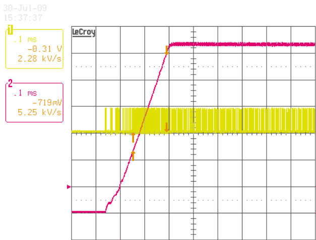
FIGURE 54. 1-PHASE GPU MODE SOFT-START, DPRSLPVR=0 , V_{IN} = 8V , I_O = 0A , V_{ID} = 1.2375V , Ch1: PHASE1, Ch2: V_O
