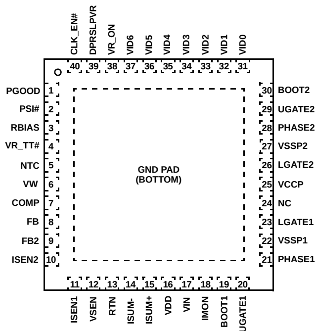
ISL62882A (40 LD TQFN) TOP VIEW
