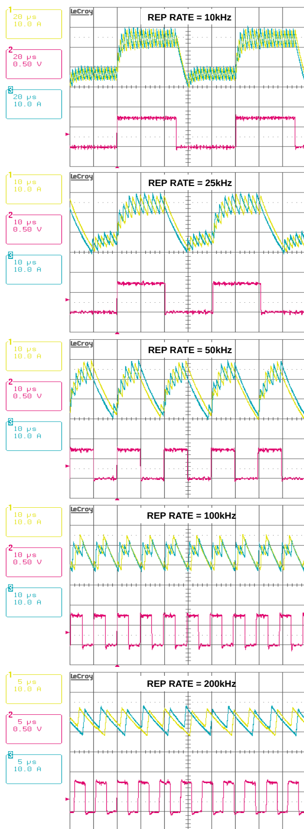
FIGURE 15. ISL62882 EVALUATION BOARD CURRENT BALANCING DURING DYNAMIC OPERATION. Ch1: IL1, Ch2: I_{load} , Ch3: IL2
