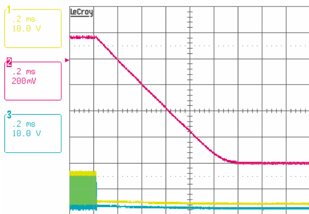
FIGURE 37. 2-PHASE CPU MODESHUT DOWN, V_{IN} = 19V , I_O = 1A , VID = 0.95V, Ch1: PHASE1, Ch2: V_O , Ch3: PHASE2
