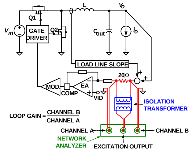
FIGURE 25. LOOP GAIN T1(s) MEASUREMENT SET-UP
