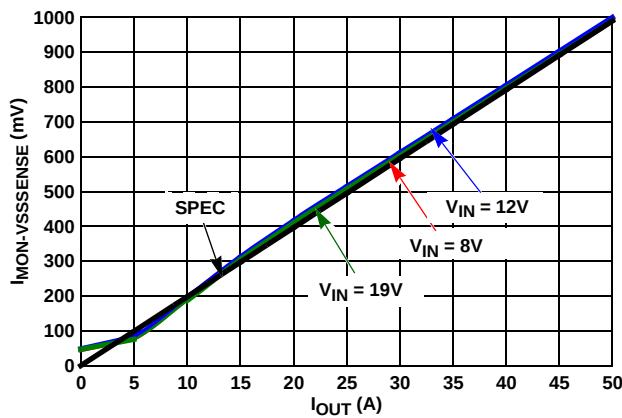
FIGURE 52. IMON, V_{ID} = 1.075
