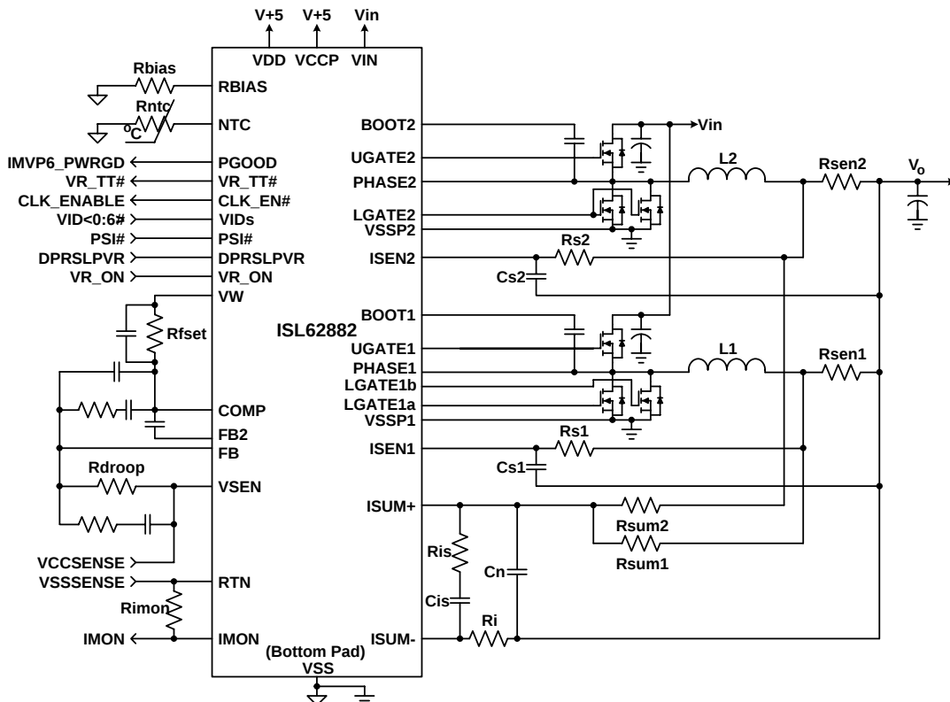
FIGURE 2. TYPICAL CPU APPLICATION CIRCUIT USING RESISTOR SENSING
