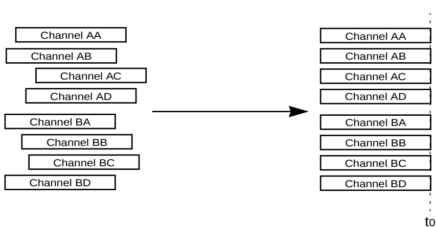
Figure 26. Alignment of all Eight SERDES Channels – ORSO82G5
