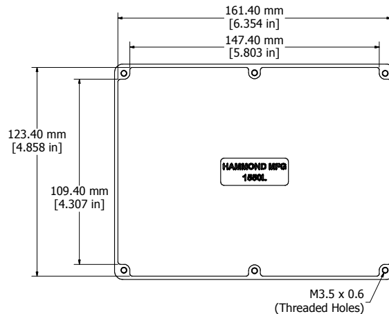
Top View Looking Inside Box
