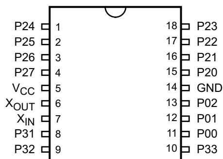
Figure 3. 18-Pin DIP/SOIC Configuration, STANDARD Mode
