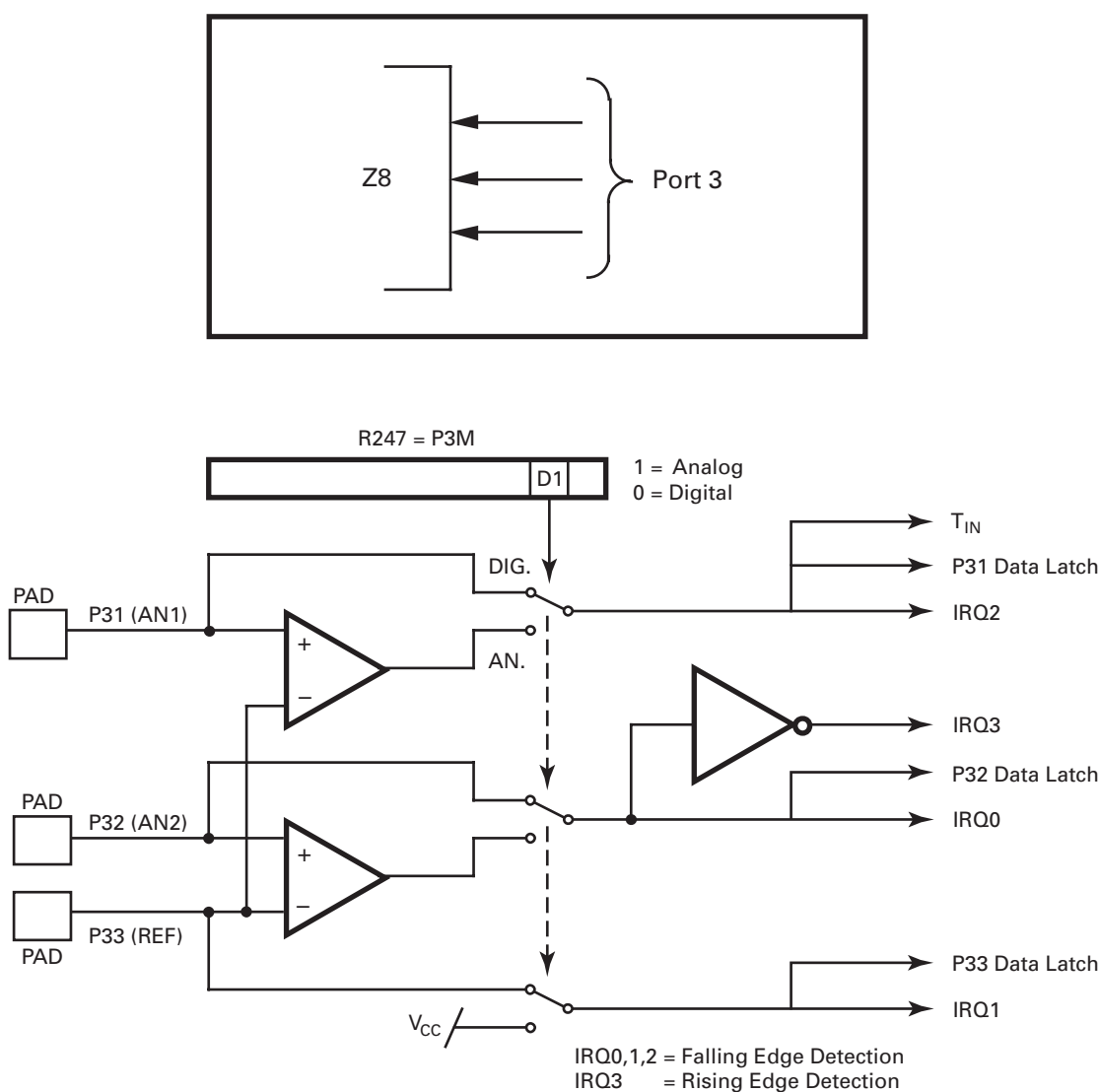
Figure 11. Port 3 Configuration
