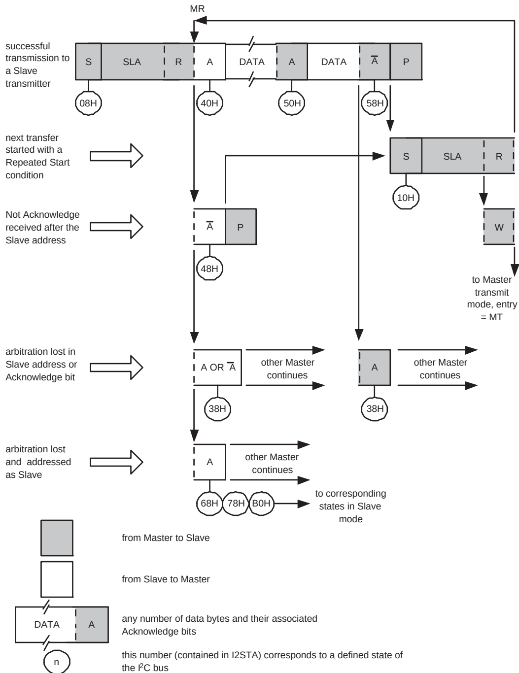
Fig 29. Format and states in Master Receiver mode
