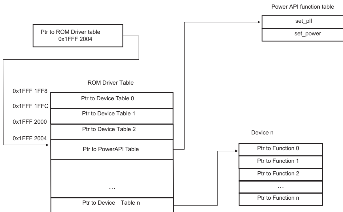
Fig 65. Power profiles pointer structure
