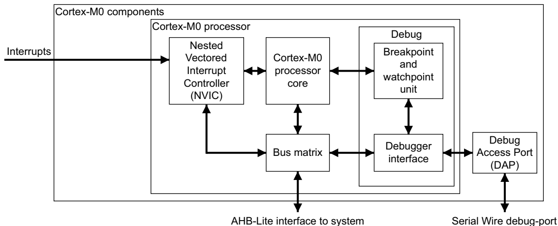
Fig 69. Cortex-M0 implementation
