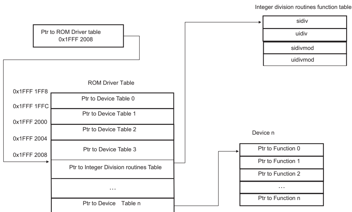
Fig 62. Integer division routines pointer structure
