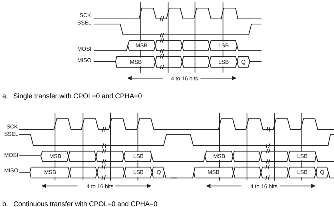
Fig 36. SPI frame format with CPOL=0 and CPHA=0 (a) Single and b) Continuous Transfer)
