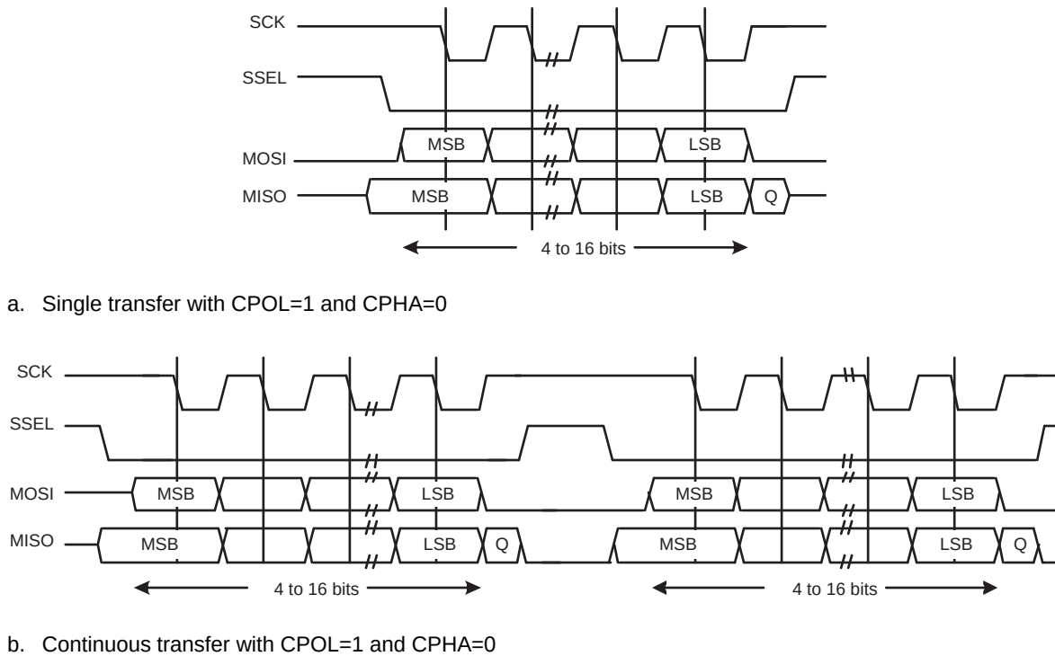
Fig 38. SPI frame format with CPOL = 1 and CPHA = 0 (a) Single and b) Continuous Transfer)
