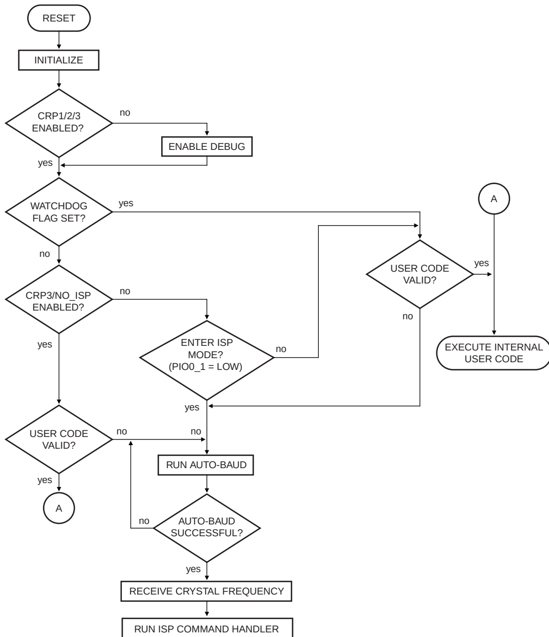
Fig 59. Boot process flowchart
