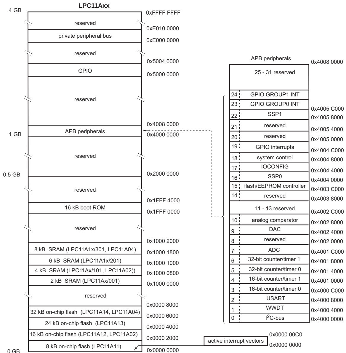
Fig 3. LPC11Axx memory map
