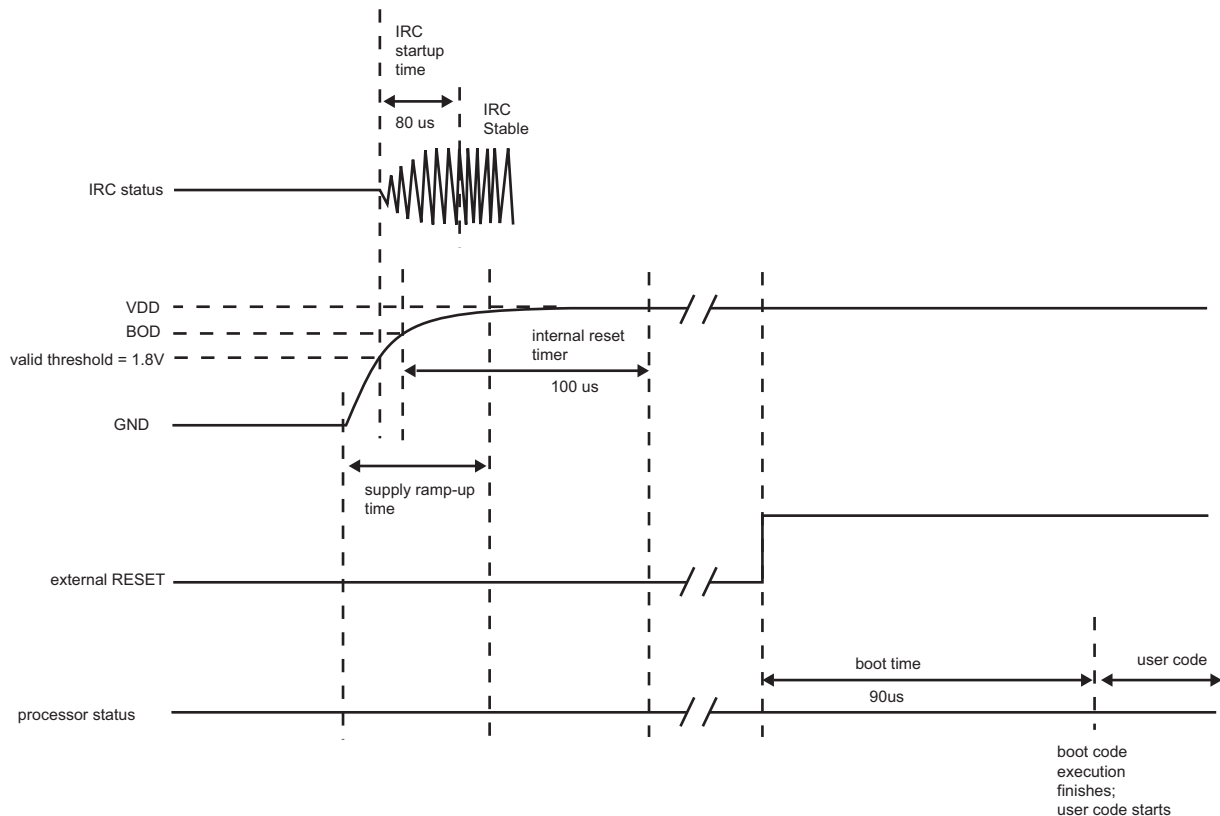
Fig 7. Typical start-up time with respect to the external reset
