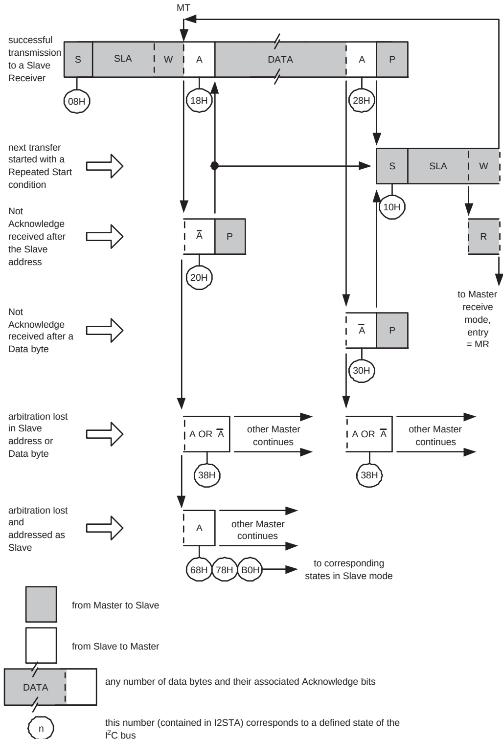
Fig 28. Format and states in Master Transmitter mode
