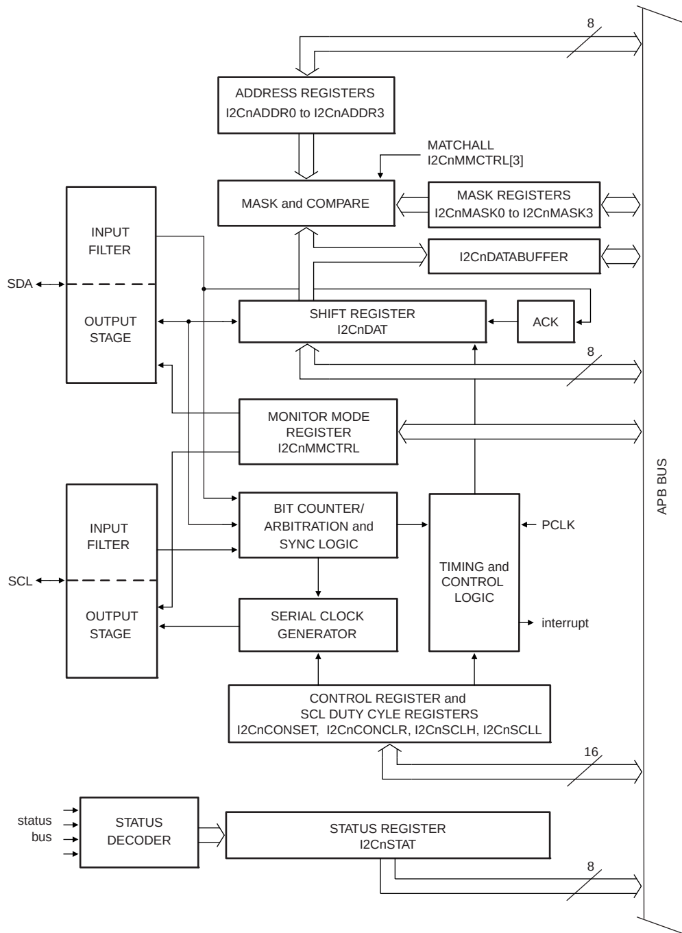
Fig 20. I 2 C serial interface block diagram
