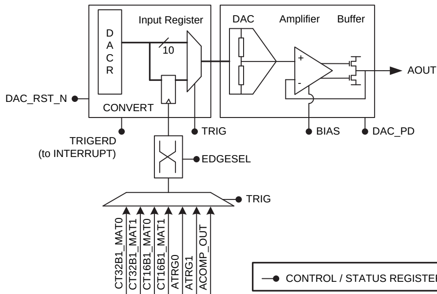
Fig 57. DAC block diagram
